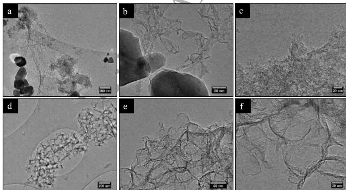
Fig. 3. Transmission electron micrographs. (a, b, c) Lobster/L, (d, e, f) Artificial Lobster/AL.
