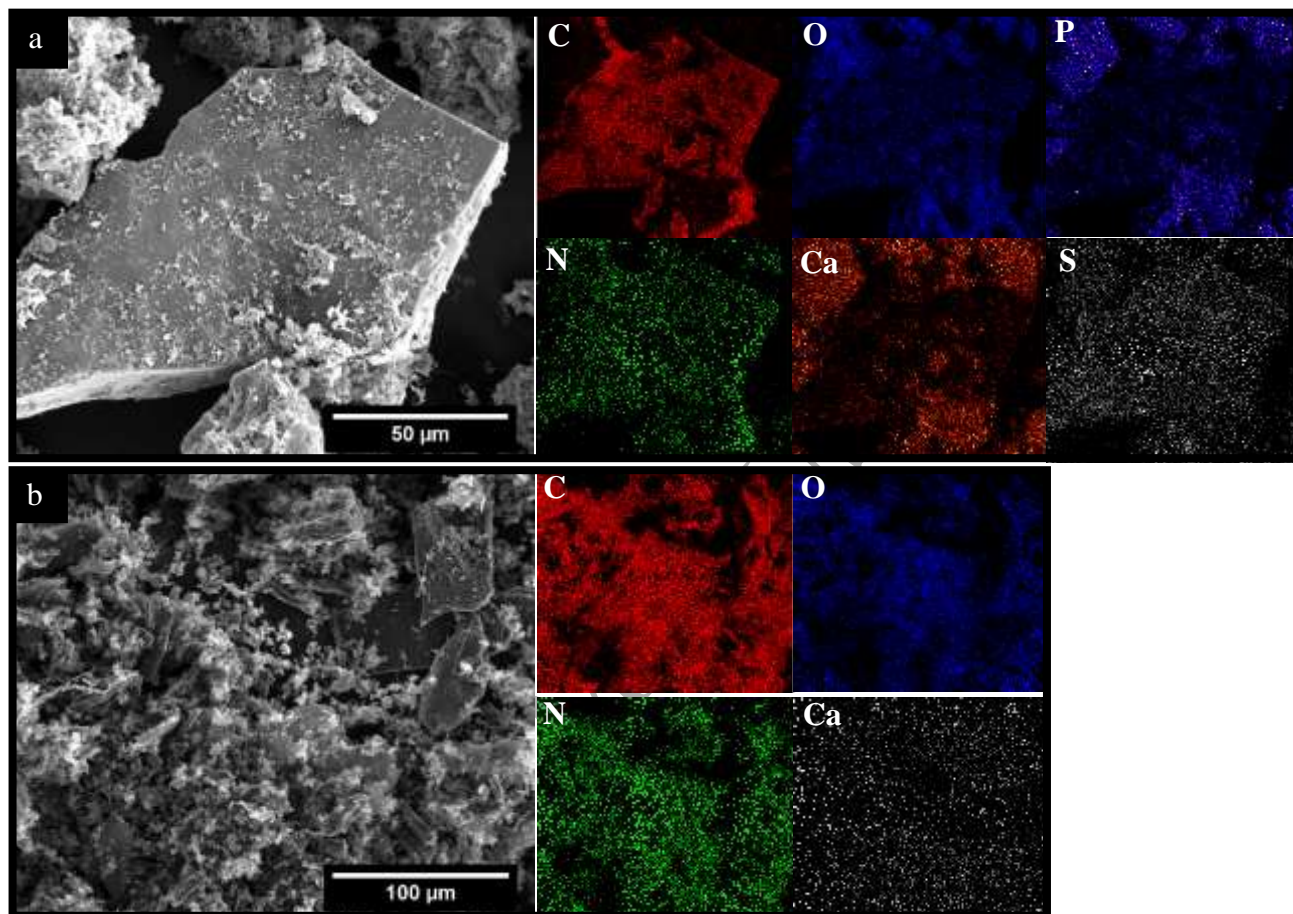
Fig. 4. Energy-dispersive X-ray spectroscopy for (a) Lobster/L showing the presence of carbon, oxygen, nitrogen, calcium, phosphorus and sulphur and (b) Artificial Lobster/AL showing carbon, oxygen, nitrogen and calcium.
