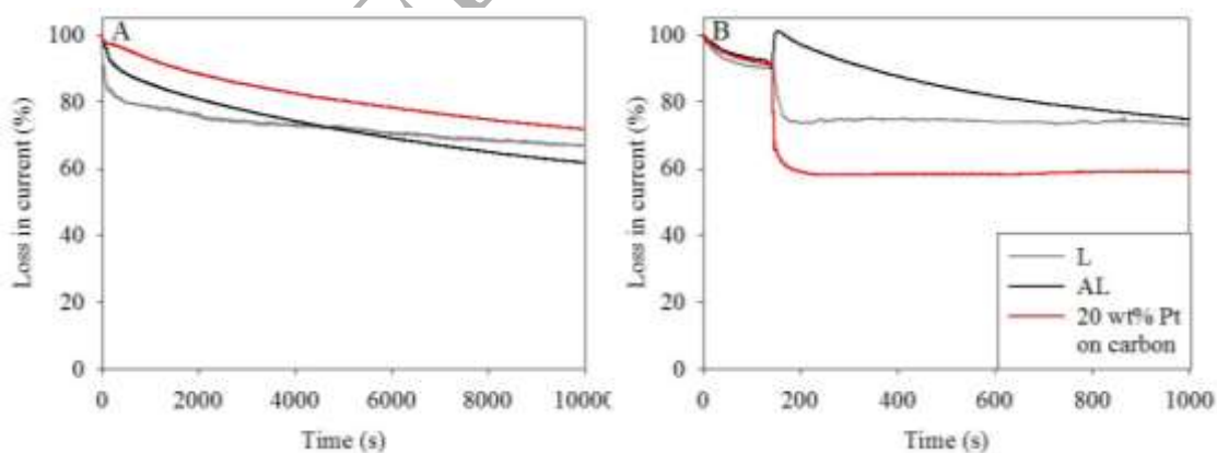
Fig. 10. Comparison of the chronoamperic response recorded at a constant rotational speed of 800 rpm and potential of -0.25 V for (a) stability testing over 10000 s and (b) methanol tolerance over 1000 s, where 5 mL of methanol was added after 160 s in 0.1 M KOH for Lobster/L (grey), Artificial Lobster/AL (black) and 20 wt% platinum on Vulcan carbon (red).
