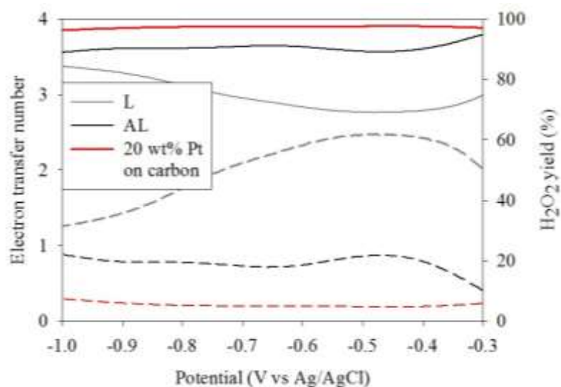
Fig. 9. Electron transfer number (full lines) and hydrogen peroxide yield (dotted lines) calculated via RRDE measurements in 0.1 M KOH for Lobster/L (grey), Artificial Lobster/AL (black) and 20 wt% platinum on Vulcan carbon (red).
