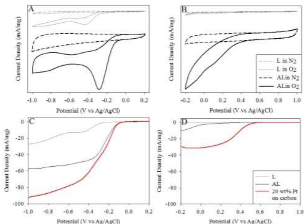
Fig. 8. Cyclic voltammograms for Lobster/L (grey) and Artificial Lobster/AL (black) in (a) 0.1 M KOH and (b) 0.5 M H 2 SO 4 either saturated with nitrogen (dotted lines) or oxygen (full lines) recorded with a RDE setup. Comparison of the RRDE polarisation curves at 1600 rpm for Lobster/L (grey), Artificial Lobster/AL (black) and 20 wt% platinum on Vulcan carbon (red) in (c) 0.1 M KOH and (d) 0.5 M H 2 SO 4 .
