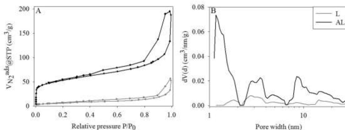
Fig. 1. (a) Nitrogen sorption isotherms and (b) pore size distribution for Lobster/L (grey) and Artificial Lobster/AL (black) after the acid treatment.
