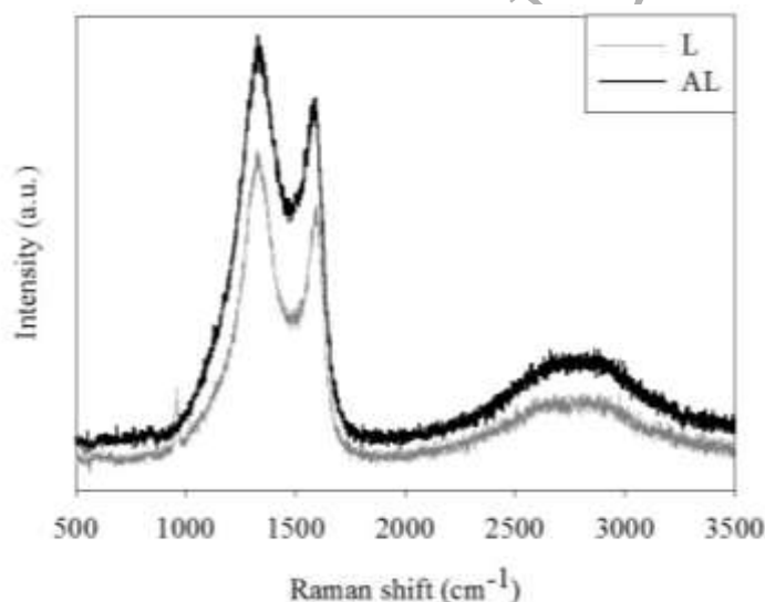
Fig. 6. Raman spectra performed at an excitation wavelength of 633 nm for Lobster/L (grey) and Artificial Lobster/AL (black).
