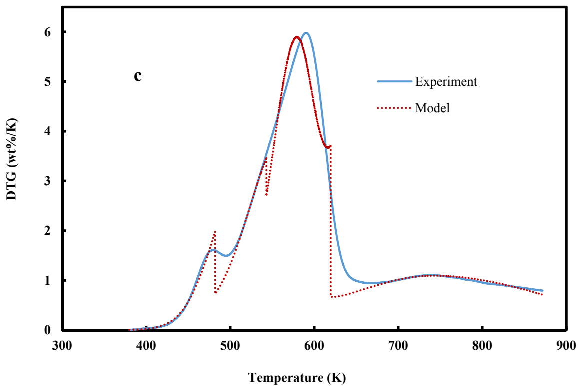
Figure 4. Comparison between Experimental and Predicted DTG curves of Napier Grass Biomass. (a) NGL; (b) NGS; (c) NGT.
