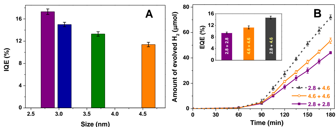
Fig. 2 A) Internal quantum efficiency for photocatalytic hydrogen generation as function of SNC diameter in single-cell geometries. B) Hydrogen evolution as a function of time for dual-band gap cells with 2.8 nm SNCs only (purple solid squares), 4.6 nm SNCs only (orange open circles), and 2.8 nm+4.6nm SNCs (black solid triangles). Inset: External quantum efficiencies for photocatalytic hydrogen evolution in the same dual-band gap geometries. (In all measurements the OD of the SNC suspensions were kept at 1.5 in each cell at the first excitonic absorption peak resulting in 26 - 53 mg/L of Pt-decorated CdS for the four sizes. Samples were excited with a power of ~50 mW/cm 2 and spectral range between 350-480 nm. SNC suspension contained 0.02 M sodium sulphite as hole scavenger and 0.05 M triethanolamine as stabiliser with at a pH of 9).
