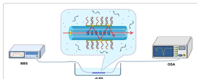
Figure 4: Experimental setup for fiber grating based biosensor sensing system. Inset: schematic diagram of hybridization process between probe oligonucleotide immobilized dLPG biosensor and complementary oligonucleotides.
