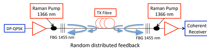
Fig. 1. Unrepeated transmission line set-up.
