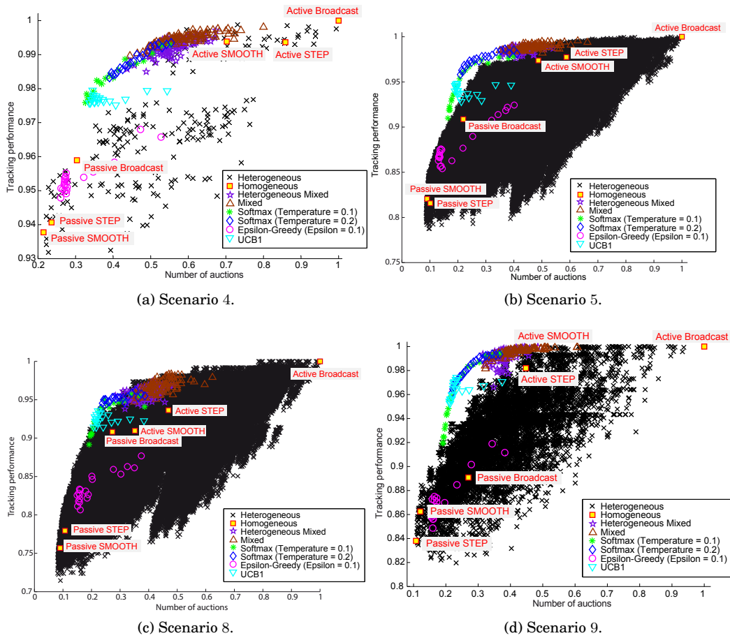
Fig. 9. Performance for scenarios 4, 5, 8 and 9, showing homogeneous and heterogeneous assignment of strategies, mixed and heterogeneous mixed strategies, and assignments done by bandit solvers. The results have been normalized by the maximum value of the ACTIVE BROADCAST strategy and are averages over 30 runs with 1000 time steps each. The bandit solvers' reward functions normalised the number of auction invitations by distribution at runtime.
