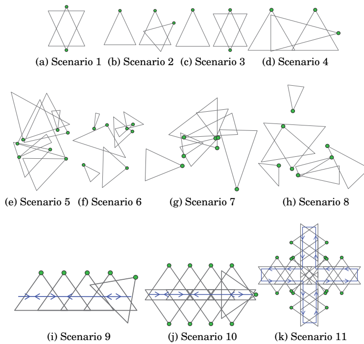
Fig. 1. The scenarios tested with our simulation tool CamSim . A dot represents a camera, the associated triangle represents its FOV. Blue arrows indicate the predefined movement paths.
