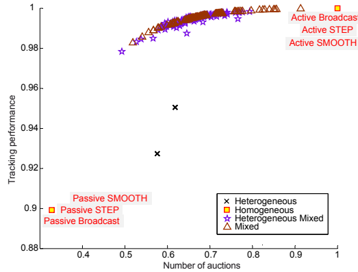
Fig. 5. Performance for scenario 1 showing homogeneous, heterogeneous, mixed and heterogeneous mixed assignment of strategies. The results have been normalized by the maximum value of the ACTIVE BROADCAST strategy and are averages over 30 runs with 1000 time steps each.
