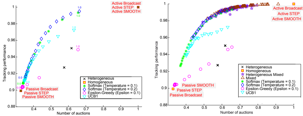
(a) Using original reward values for bandit solvers. (b) Using reward values normalised by distribution.
