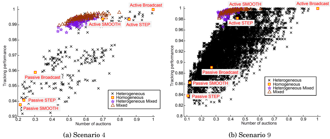
Fig. 6. Performance for scenario 4 and scenario 9 showing homogeneous, heterogeneous, mixed and meta-mixed assignment of strategies. The results have been normalized by the maximum value of the ACTIVE BROADCAST strategy and are averages over 30 runs with 1000 time steps each.
