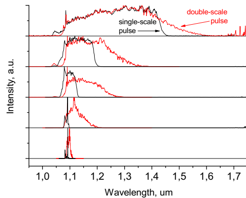
Fig. 6. Raman radiation spectra from 1.2-km long phosphosilicate fiber pumped with single-scale (black curves) and double-scale (red curves) pulses. (For interpretation of the references to colour in this figure legend, the reader is referred to the web version of this article.)
