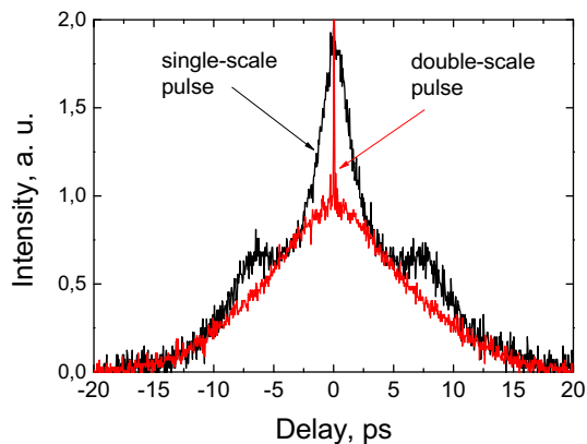
Fig. 5. Auto-correlation functions of single-scale (black curve) and double-scale (red curve) pulses used in the experiment. (For interpretation of the references to colour in this figure legend, the reader is referred to the web version of this article.)
