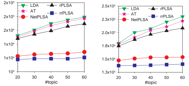
(a) \mathcal{D}_{music} (b) \mathcal{D}_{random} Fig. 4. Performance comparisons of perplexity on Twitter datasets.
