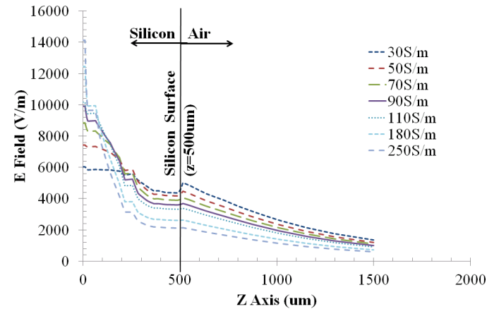
Fig. 18. E-field (Magnitude) distribution across the centre of the plasma for multilayer layer model in the z direction at 10 GHz.
