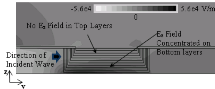
Fig. 19. E_z field contours for inhomogeneous multilayer plasma at 10 GHz this shows the TEM mode of propagation at the lower frequencies.
