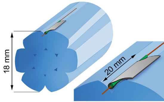
Fig. 3. Diagram of a capillary-encapsulated fibre Bragg grating (FBG) attached to a prestressing strand
