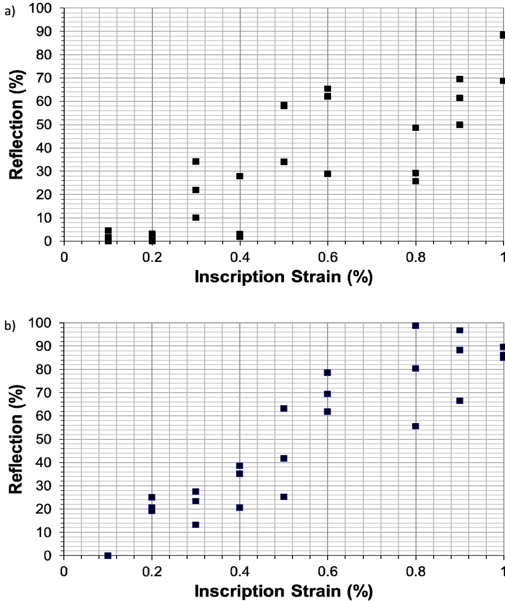
Figure 2 Bragg reflection against inscription strain (a) grating pitch of 278.75 nm (b) grating pitch 530.59 nm
