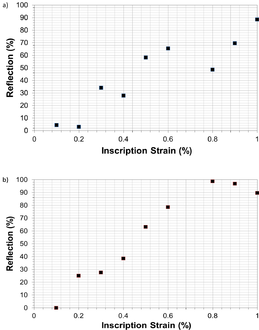
Figure 3 Maximum values of Bragg reflection against inscription strain (a) grating pitch of 278.75 nm (b) grating pitch 530.59 nm
