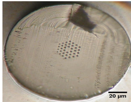
Figure1 Transversal section of the microstructured polymer optical fibre.
