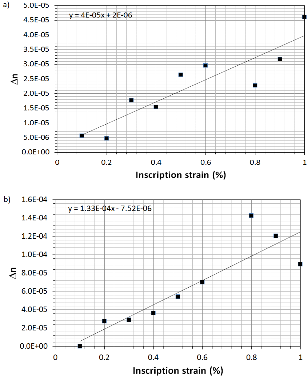
Figure 4 Refractive index Modulation against inscription strain. (a) grating pitch of 278.75 nm, (b) grating pitch of 530.59nm.
