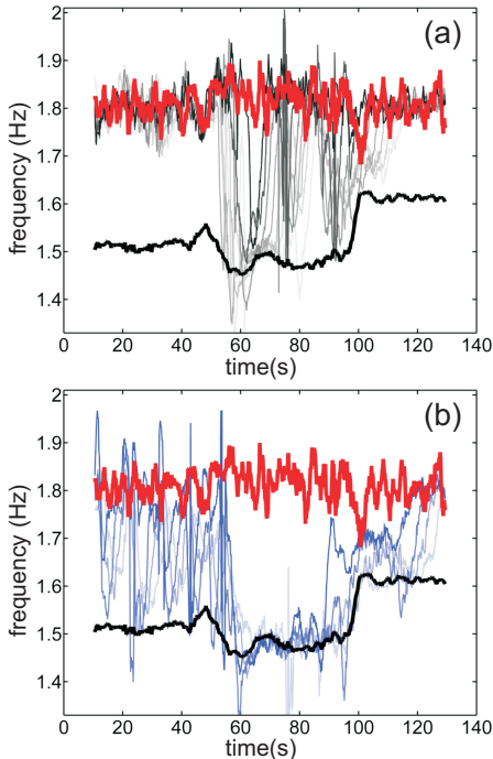
FIG. 5: Frequency analysis of the data shown in Fig. 4 (color online). (a) Thick red curve: frequency of the pacemaker, thick black curve: frequency far away from the target pattern (natural frequency), the curves in different shades of gray indicate the frequency at distances of four (dark gray) to ten (light gray) \lambda from the pacemaker along the white line in Fig. 4 (a). (b) Blue lines indicate the frequency at distances of 11 (dark blue) to 14 (light blue) \lambda from the pacemaker.
