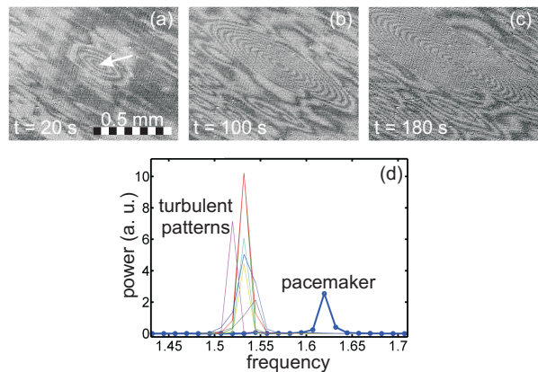
FIG. 2: Suppression of turbulence by a laser induced target pattern (color online). (a)-(c) Snapshots at indicated time moments after initiation of the laser spot. (d) Frequency spectrum at the center of the target pattern compared to frequency of the background dynamics. The white arrow in (a) indicated the position of the laser spot. The reaction parameters are P_{\text{Laser}} = 49 mW, p_{\text{O}_2} = 1.84 \times 10^{-4} mbar, p_{\text{CO}} = 7.84 \times 10^{-5} mbar, and T = 538 K.
