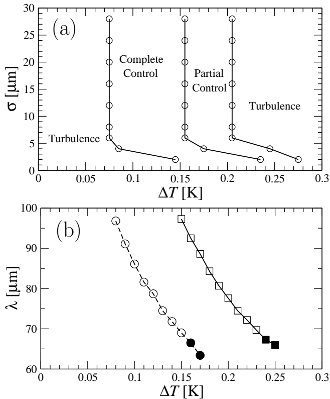
FIG. 7: Analysis of patterns induced by the pacemaker. (a) Control diagram. Depending on the choice of parameters \Delta T (temperature shift) and \sigma (size of the heterogeneity) we find regions of partial and complete control. (b) Wavelength of the generated target patterns as a function of temperature shift for \sigma = 2 \mu\text{m} (solid curve) and \sigma = 24 \mu\text{m} (dashed curve). Solid symbols indicate simulations that lie in the regime of partial control.
