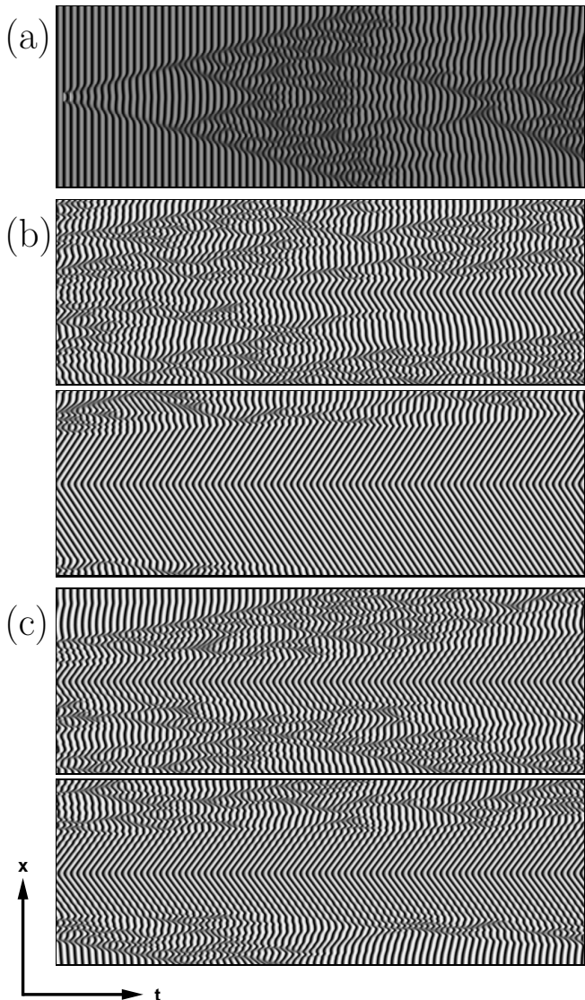
FIG. 6: Spatiotemporal dynamics in the KEE model. Parameters: T_0 = 543.5 K, p_{\text{CO}} = 4.46 \times 10^{-5} mbar, and p_{\text{O}_2} = 1.1 \times 10^{-4} mbar. Shown are space-time diagrams in gray scale for u . Black (white) denotes minimum (maximum) values of u in the shown simulation. (a) Development of intermittent turbulence from an initial perturbation (strong, momentary, localized increase of u in the center of the medium). System size is L = 800 \mu\text{m} , shown time interval t = [0, 200] s. (b) Complete control: full suppression of turbulence by a heterogeneous pacemaker ( \Delta T = 0.13 K, \sigma = 16 \mu\text{m} ). System size is L = 1400 \mu\text{m} , heterogeneity is switched on at t = 0 s. Shown are time intervals t = [200, 400] s (upper panel) and t = [839, 1039] s (lower panel). (c) Partial control: spatially confined suppression of turbulence by a heterogeneous pacemaker ( \Delta T = 0.17 K, \sigma = 16 \mu\text{m} ). System size is L = 1400 \mu\text{m} , heterogeneity is switched on at t = 0 s. Shown are time intervals t = [200, 400] s (upper panel) and t = [1300, 1500] s (lower panel).
