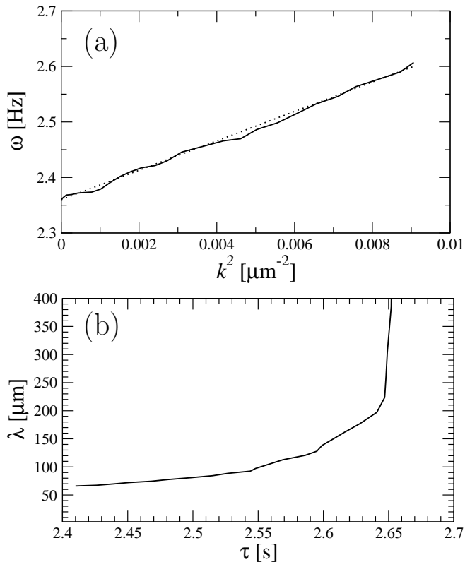
FIG. 9: Dispersion relations \omega(k^2) (a) and \lambda(\tau) (b). A linear fit to \omega = \omega(k^2) (dotted curve) is added.
