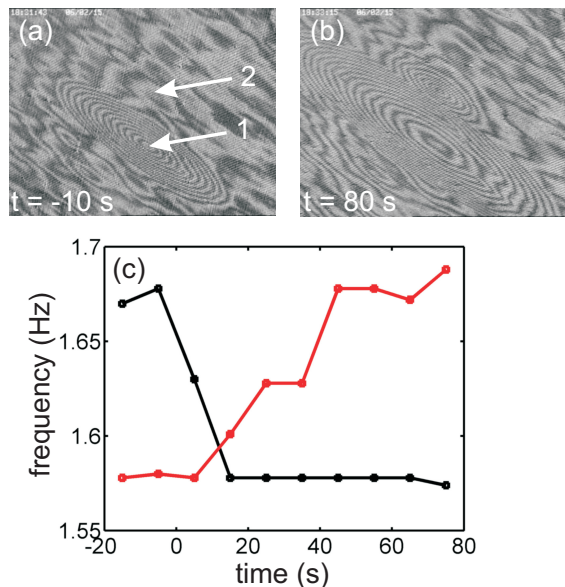
FIG. 3: Moving the laser spot (color online). (a) Snapshot 10 s prior to move, arrows indicate old (1) and new (2) position of the laser spot, (b) snapshot 80 s after move, (c) frequency evolution at the old (black) and the new (red) location of the laser spot. The reaction parameters are P_{\text{Laser}} = 53 mW, p_{\text{O}_2} = 1.84 \times 10^{-4} mbar, p_{\text{CO}} = 7.84 \times 10^{-5} mbar, and T = 538 K.
