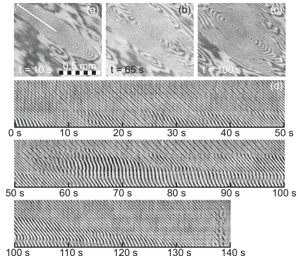
FIG. 4: Partial control (color online). (a-c) snapshots of the system at indicated time moments. (d) space-time-plots along the line indicated in (a). After the oxygen pressure is decreased from 2.064 \times 10^{-4} mbar to 2.058 \times 10^{-4} mbar at t = 45 s, the target pattern collapses via a cascade of phase slips. The reaction parameters are P_{\text{Laser}} = 63 mW, p_{\text{CO}} = 8.40 \times 10^{-5} mbar, T = 539 K, p_{\text{O}_2} = 2.068 \times 10^{-4} mbar for t > 95 s.
