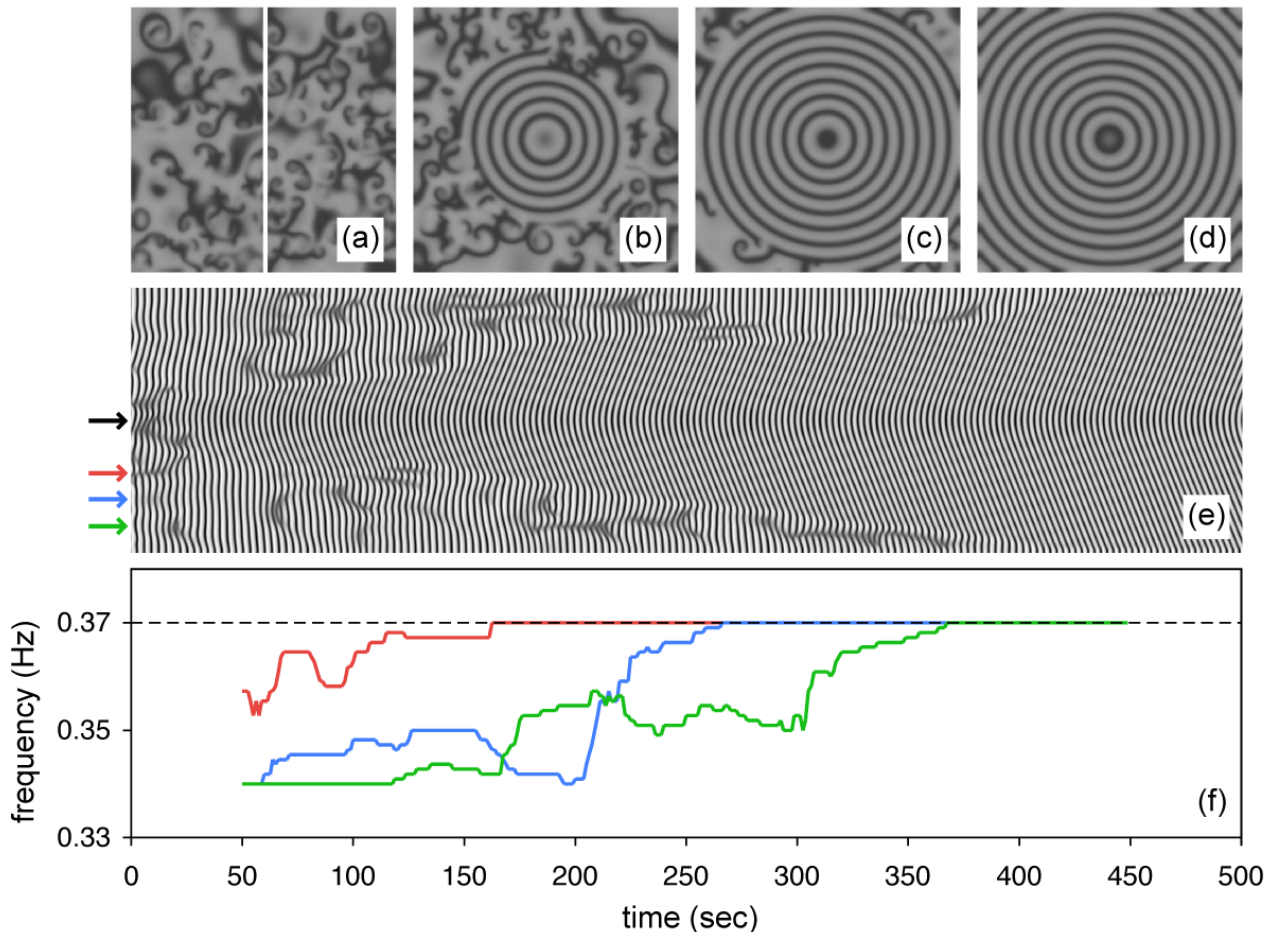
FIG. 10: (Color online) Control of chemical turbulence in a two-dimensional system by a temperature induced pacemaker. A temperature heterogeneity of Gaussian shape ( \Delta T = 0.3 K and \sigma = 40 \mu\text{m} ) is induced at t = 0 s in the center of the domain. The partial pressures of the reactants are p_{\text{CO}} = 4.46 \times 10^{-5} mbar and p_{\text{O}_2} = 10.6 \times 10^{-5} mbar, the base temperature is T_0 = 543.5 K. (a) Chemical turbulence at time t = 0 s. Emerging target pattern at (b) t = 250 s, (c) t = 500 s, and (d) t = 750 s. (e) Space-time diagram along the vertical white line indicated in (a); time axis as in (f). (f) Frequency analysis of time series at four different points in space indicated by colored arrows on the left hand side of the space-time diagram (e), the dashed black line showing the frequency in the center of the pacemaker.
