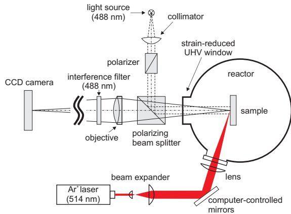
FIG. 1: Experimental setup (color online). Upon reflection at the platinum surface (sample) the light changes polarization because the Pt(110) surface is optically anisotropic. When covered with CO, the optical properties of the crystal surface change slightly compared to a clean or oxygen covered surface. This is visualized using the polarizing beam splitter cube which acts as a filter. Light reflected from reactive surface areas is blocked, but light reflected from surface regions covered with CO can pass. The platinum surface is imaged onto the chip of a CCD camera using a simple achromatic lens. The light of an Ar-ion laser is focused onto the surface and can be positioned via computer controlled mirrors. Reproduced from [49].
