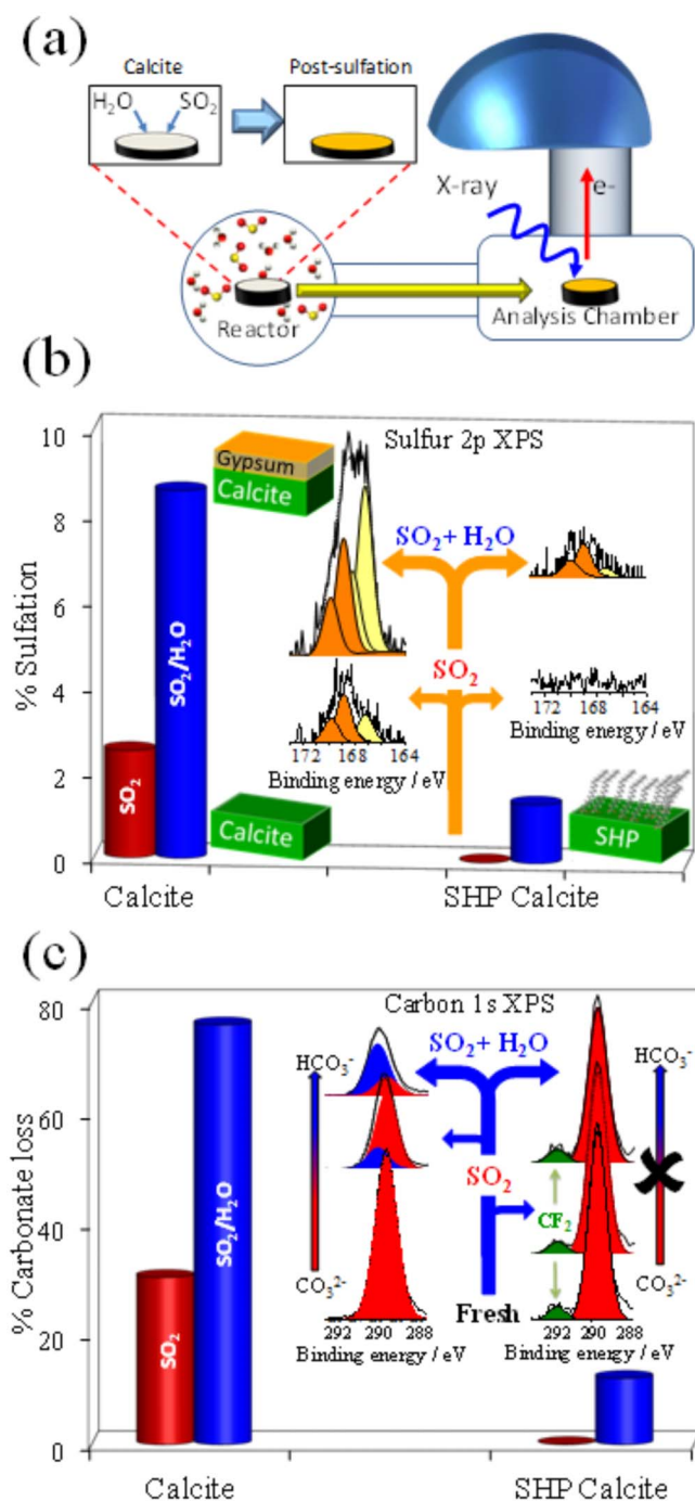
Figure 2 | In-situ XPS of calcite and SHP-calcite surfaces following in-situ exposure to SO 2 or 100 mTorr SO 2 + 18 Torr H 2 O for 18 h.
