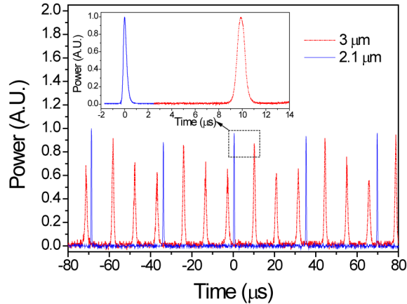
Fig. 4. Synchronized output pulse trains for the Q-switched {}^5I_7 \rightarrow {}^5I_8 pulse and gain-switched {}^5I_6 \rightarrow {}^5I_7 pulse for the maximum launched pump power of 7.4 W. The inset shows the temporal pulse waveform for {}^5I_6 \rightarrow {}^5I_7 and {}^5I_7 \rightarrow {}^5I_8 transitions.
