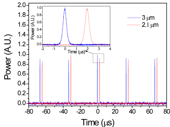
Fig. 2. Synchronized output pulse trains for the Q-switched {}^5\text{I}_6 \rightarrow {}^5\text{I}_7 pulse and the gain-switched {}^5\text{I}_7 \rightarrow {}^5\text{I}_8 pulse at the repetition rate of 30 kHz for the maximum launched pump power of 7.4 W. The inset shows the temporal pulse waveform for {}^5\text{I}_6 \rightarrow {}^5\text{I}_7 and {}^5\text{I}_7 \rightarrow {}^5\text{I}_8 transitions.
