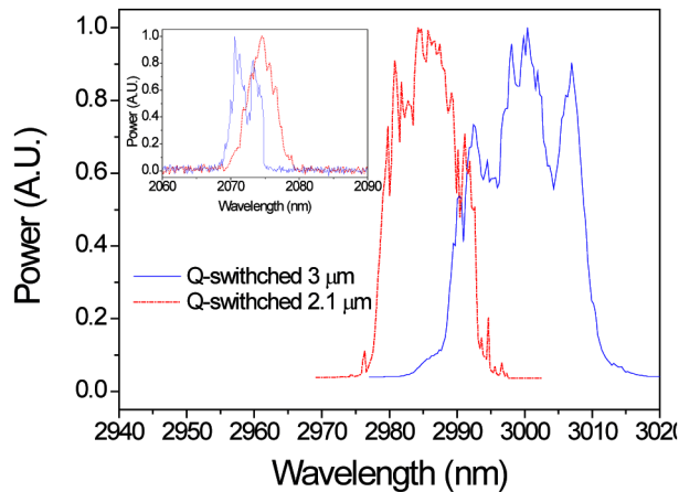
Fig. 5. Measured spectrum of the {}^5I_6 \rightarrow {}^5I_7 laser transition at maximum pump power. The inset shows the measured spectrum for the {}^5I_7 \rightarrow {}^5I_8 laser transition at maximum pump power.
