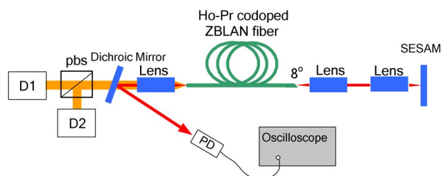
Fig. 1. (Color online) Schematic of the experiment setup. D1-D2 represents the pump diodes, pbs represents the polarizing beam splitter, and PD represents the photodetector.
