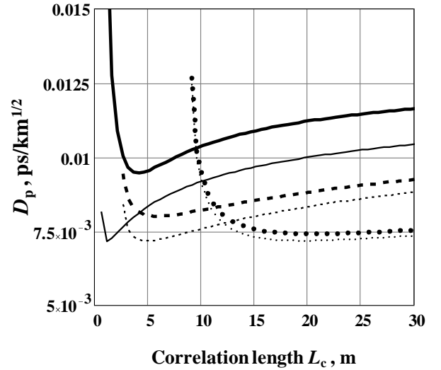
Figure 3. PMD parameter D_p as a function of correlation length L_c in the two-section fiber according to Eqs. (1,3,4-6) for D_p^{(1)} = 0.05 \text{ ps}\cdot\text{km}^{-1/2} (solid line), D_p^{(1)} = 0.1 \text{ ps}\cdot\text{km}^{-1/2} (dotted line), and D_p^{(1)} = 0.2 \text{ ps}\cdot\text{km}^{-1/2} (dashed line), calculated with the help of Eqs. (1,3,4-6) (thin lines) and with the help of Eqs. (1,3,5-6) (thick lines). Parameters: L=50 \text{ km} , \alpha_s=0.2 \text{ dB/km} , \lambda_p=1460 \text{ nm} , \lambda_s=1550 \text{ nm} , g=2.3 \text{ W}^{-1}\text{km}^{-1} , P=0.5 \text{ W} .
