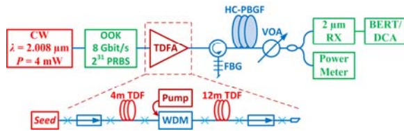
Fig.4: Experimental set-up and zoomed-in scheme of the custom-built TDFA.
