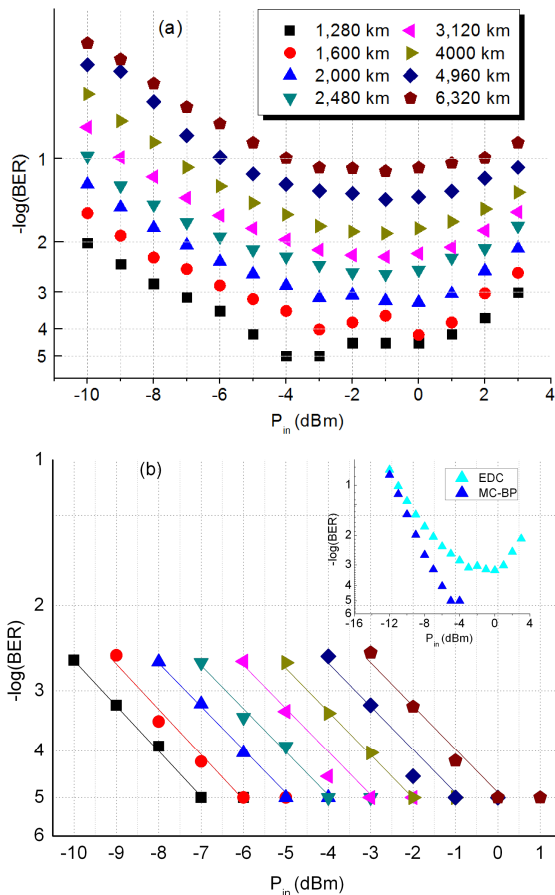
Fig. 2 BER of a nine-channel 112 Gb/s PM-4QAM transmission system without inline optical dispersion compensation as a function of launch power per channel per span. We plot various transmission reaches for (a) EDC alone for residual dispersion compensation and (b) MC-BP. Also shown in the inset is a direct comparison of the performance of the two compensation strategies after 2,000 km.
