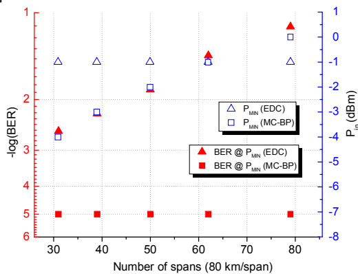
Fig. 3 Minimum achievable BER (left axis, red) and required P_{\text{min}} per channel per span, observed for the given system (right axis, blue) versus number of fibre spans by using EDC alone (triangles) and full-bandwidth back-propagation (squares) for a system without inline optical dispersion compensation (PM-4QAM).
