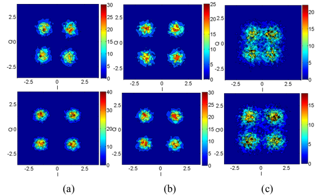
Fig. 6 Constellation diagrams after single-channel (top) and full-bandwidth (bottom) back-propagation of a nine-channel 112 Gb/s/channel PM-4QAM transmission system after 6,320 km a) for dispersion maps with 0% inline compensation; b) 50% inline compensation; c) 100% inline compensation.
