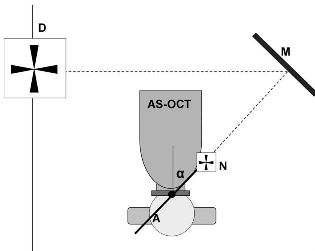
FIGURE 1. Schematic diagram of the laboratory setup for imaging nasal ciliary muscle using the AS-OCT. The subject views a near Maltese cross (N) at either -4.0 - or -8.0\text{-D} stimulus vergence, attached to an adjustable apparatus (A) mounted on the AS-OCT headrest. Angle \alpha = 40^\circ . The relaxed ciliary muscle is imaged by removing the near target from the apparatus, allowing the subject to view, via a mirror (M), a distant maltese cross (D) positioned on the laboratory wall, resulting in a stimulus vergence of -0.19 D. For clarity, the mirror and distant target used for imaging temporal ciliary muscle have been omitted from the diagram, although these were present throughout the investigation.
