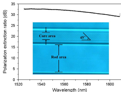
Fig. 2. (Color online) Spectral polarization extinction ratio over wavelength range from 1530 nm to 1608 nm. Inset: microscopic image of 45°-TFG structure in a PM fiber.
