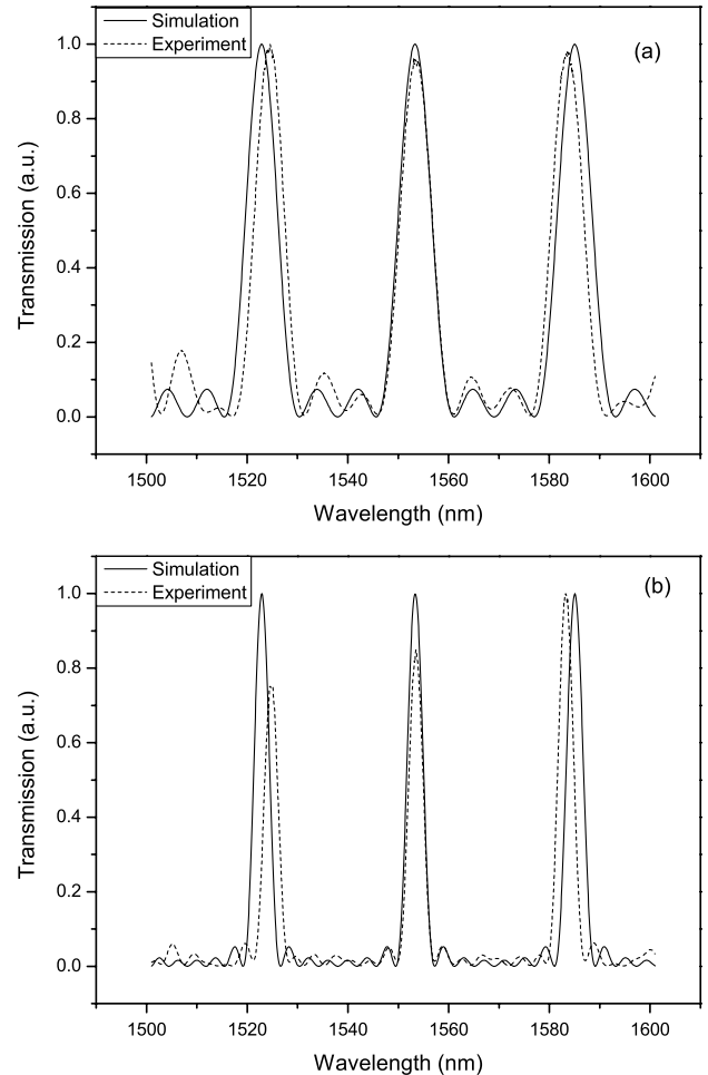
Fig. 5. Simulated (solid) and experimentally measured (dash) comblike transmission spectra of (a) 2-stage Lyot filter with PM fiber cavity length ratio 1:2 (20 cm and 40 cm) and (b) 3-stage Lyot filter with ratio 1:2:4 (20 cm, 40 cm, and 80 cm).
