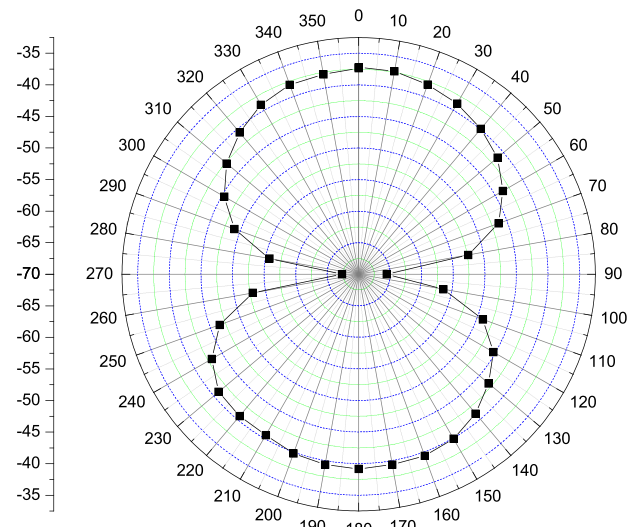
Fig. 3. (Color online) Polarization distribution of one of the 45°-TFGs UV-inscribed in PM fiber.
