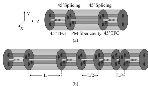
Fig. 1. (a) Configuration of an all-fiber Lyot filter using two 45°-TFGs and a PM fiber cavity. (b) Configuration of an all-fiber 3-stage Lyot-Öhman filter using four 45°-TFGs with three PM fiber cavities at a ratio 4:2:1.
