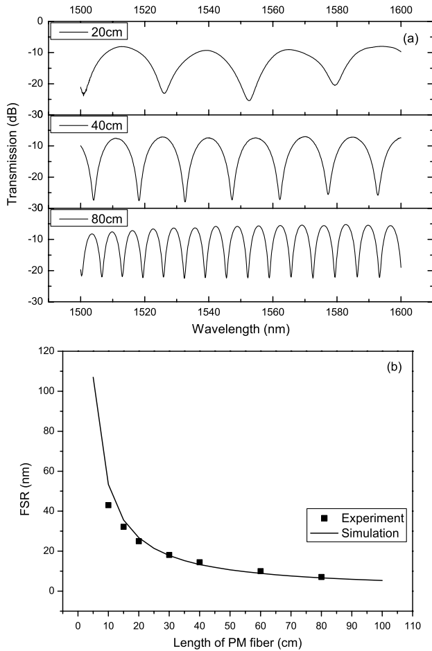
Fig. 4. (a) Measured transmission spectra of three 45^\circ -TFG based all-fiber Lyot filters with 20 cm, 40 cm, and 80 cm cavity length. (b) Experimentally measured and theoretically calculated the relationship between FSR of the filter and the length of PM fiber cavity.
