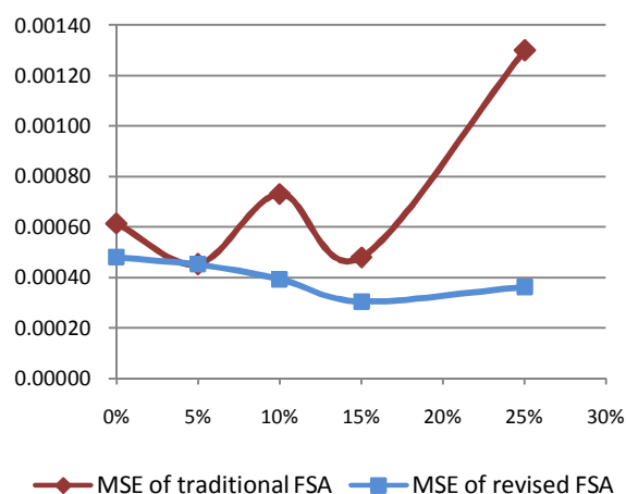
Figure 18. MSE with CRS technology, N=100
