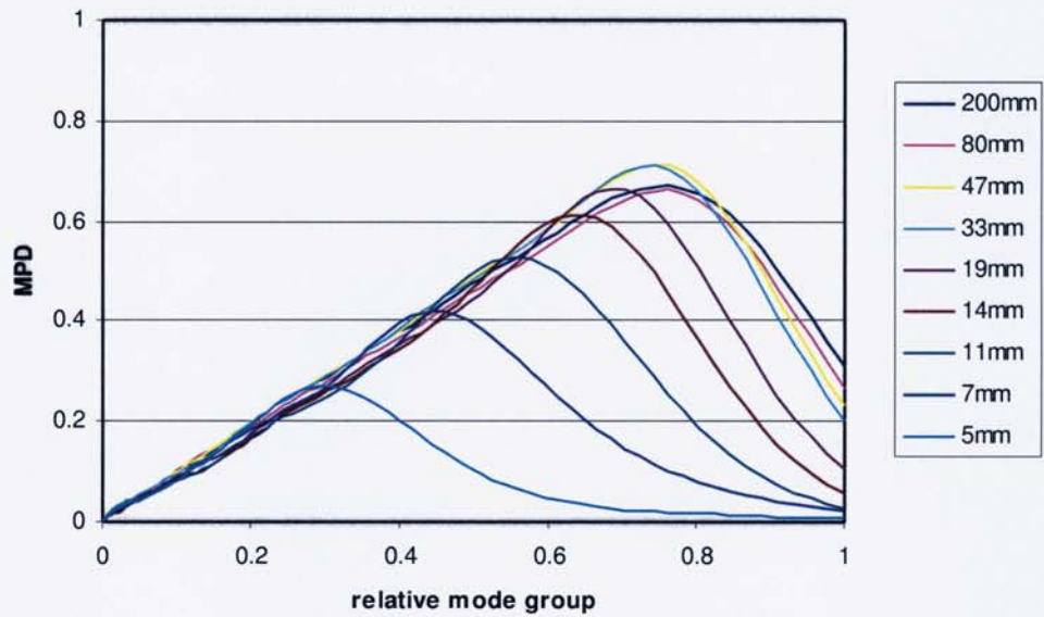
Figure 5.34. Un-normalised MPD of 50um graded-index fibre vs bend diameter of single-turn mandrel-wrap mode-filter.
