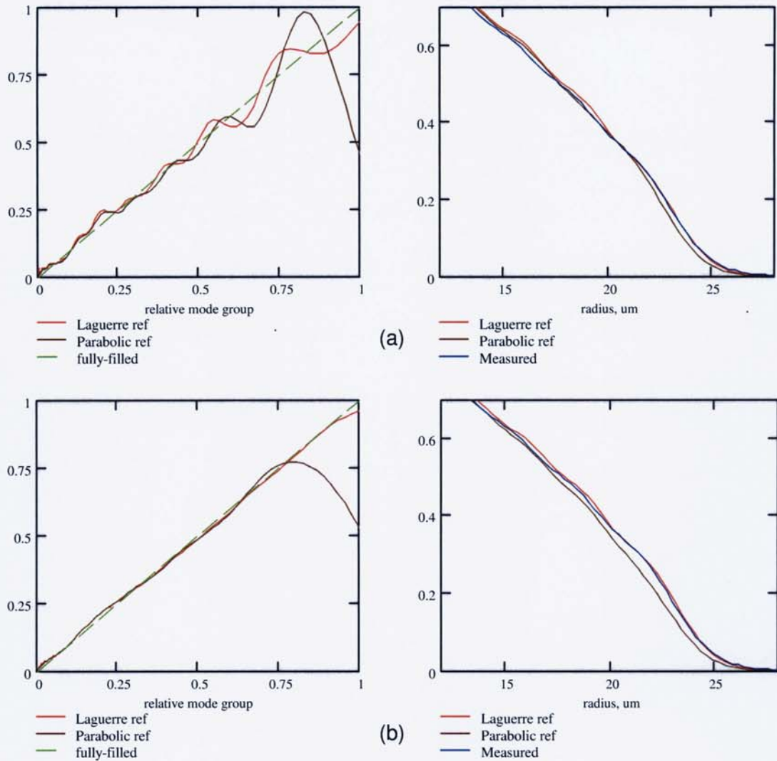
Figure 4.24. MPD of fully-filled fibre computed with Laguerre and parabolic reference profiles (left) and reconstructed near-field profiles (right) for filter widths (a) 2.7μm and (b) 7.5μm.
