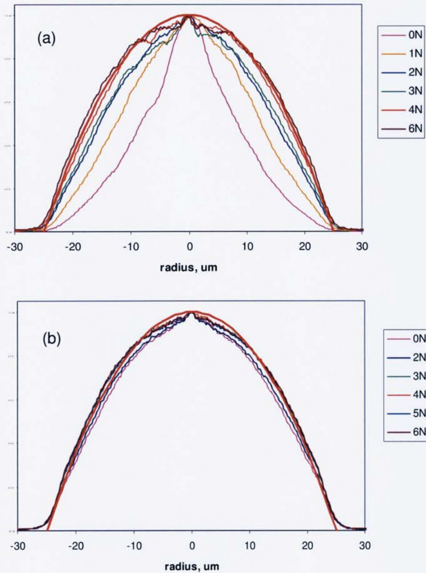
Figure 5.23. Near-field profiles of a 50µm graded-index fibre connected to step-index point-load mode-scrambler vs load for (a) singlemode launch, and (b) multimode launch. The red parabolic curve approximates a fully filled distribution.
