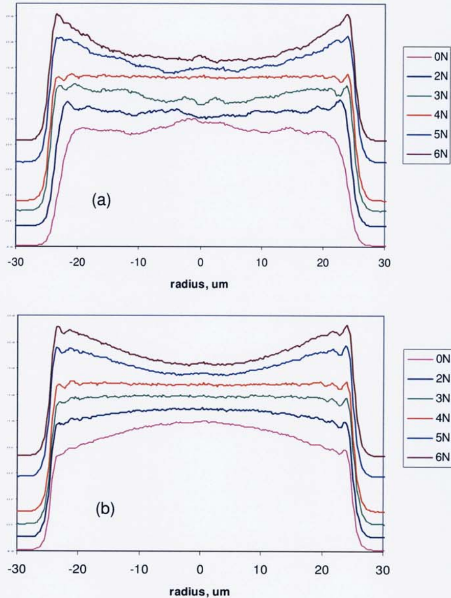
Figure 5.22. Near-field profiles of a 50µm step-index fibre with point-load mode-scrambler vs load for (a) singlemode launch, and (b) multimode launch.
