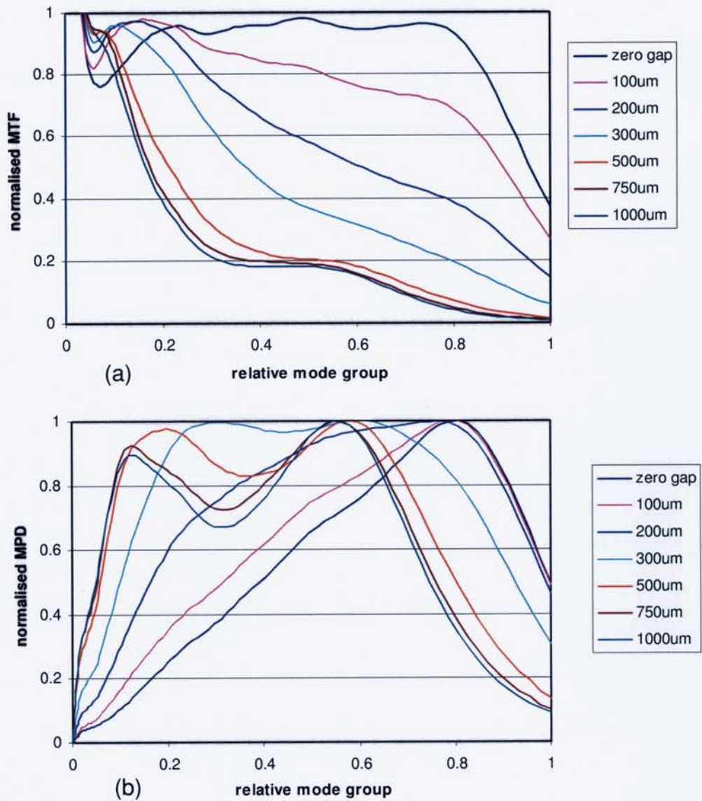
Figure 5.25. Measurement of a 50µm graded fibre spliced to a step-index fibre with an air gap vs gap width, (a) MTF, (b) MPD.
