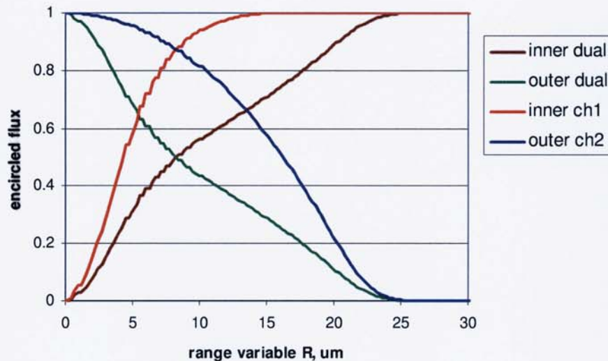
Figure 6.33. Plot of encircled flux for inner and outer regions of dual channels, and separately for ch1 (sm) and ch2 (mm), vs range variable R, for MGDM system.
