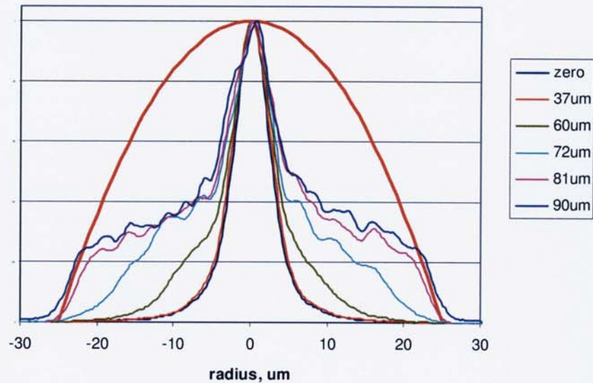
Figure 5.8. Near-field profiles of a 50μm graded-index fibre in Newport FM-1 device vs position of jaws. The red parabolic curve represents a fully-filled distribution.
