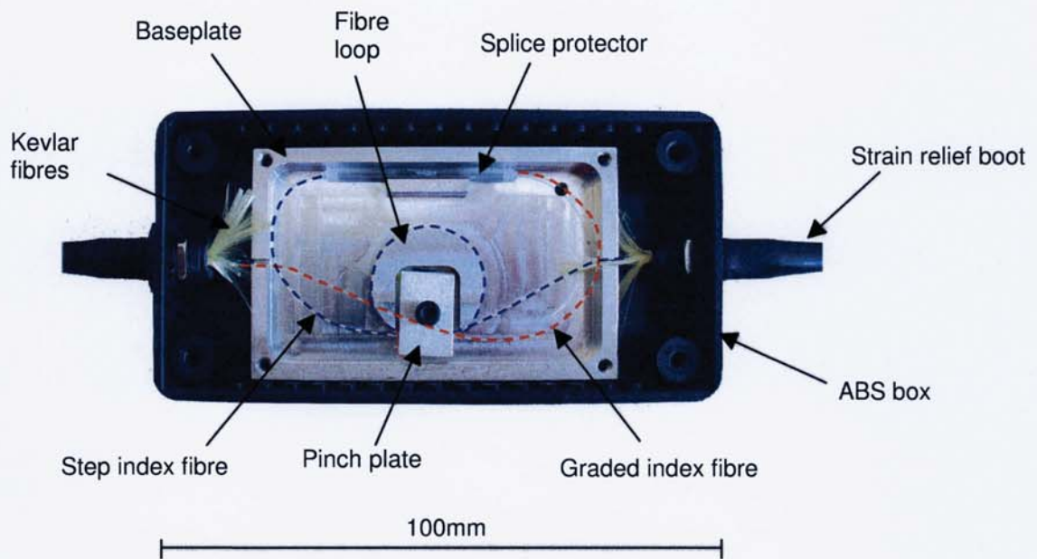
Figure 7.1. Photograph of inside of mode controller package, prior to potting.
