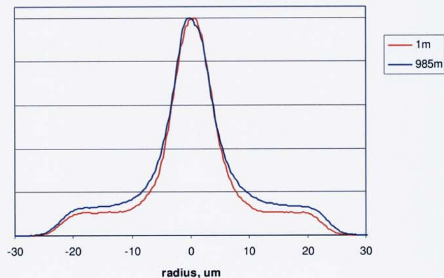
Figure 6.31. Near-field profiles of MGDM after 1m and 985m in 62.5 \mu\text{m} graded-index fibre.
