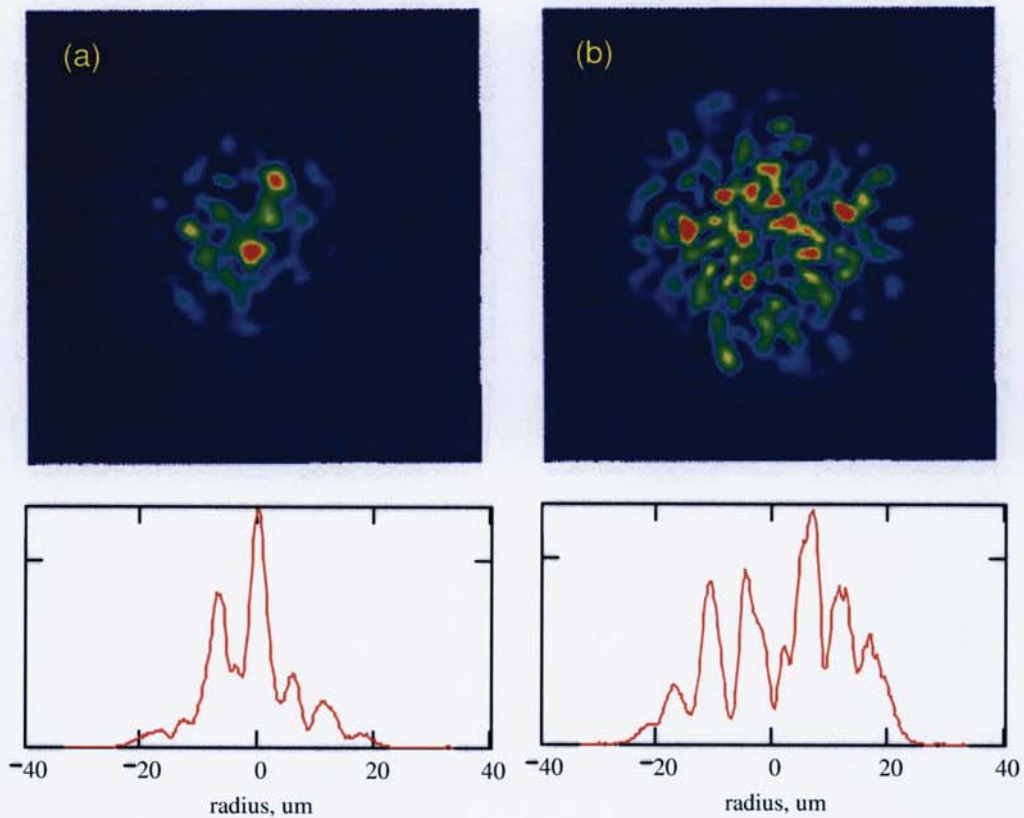
Figure 6.21. Near-field image of 50µm fibre with (a) VCSEL source, and (b) VCSEL source with mode scrambler.
