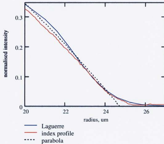
Figure 4.28. Comparison of near-field Laguerre model (blue), with the measured index profile (red), and a parabolic profile (black).
