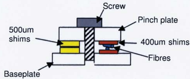
Figure 7.2. Schematic of the point loading mechanism in the mode control device.
