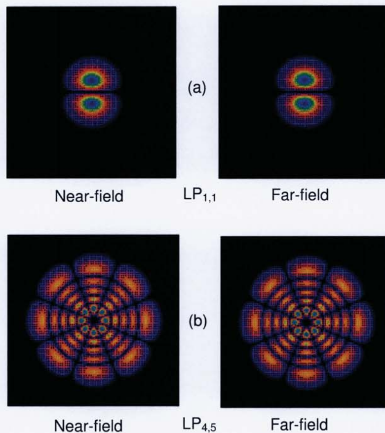
Figure 4.15. Computed near-field and far-field intensity distributions of (a) \text{LP}_{1,1} , and (b) \text{LP}_{4,5} modes in a graded-index fibre.
