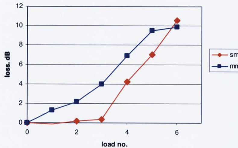
Figure 5.21. Insertion loss of a 50µm graded-index fibre with point-load mode scrambler vs load number. Red is singlemode launch and blue is multimode launch.
