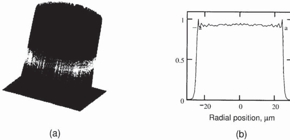
Figure 3.5. Power distribution of all guided modes, equally weighted, in 50µm core diameter step-index fibre, (a) 3-D model, (b) intensity profile.
