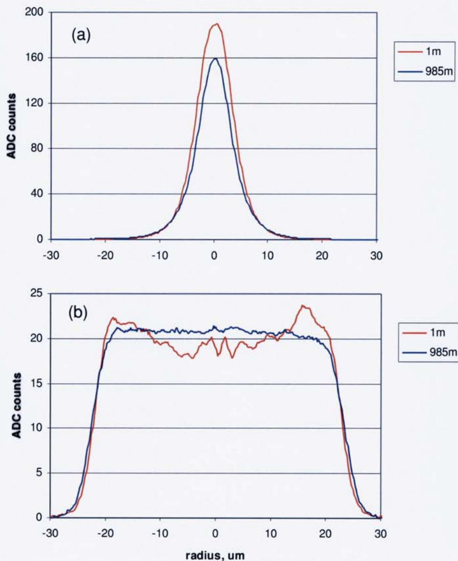
Figure 6.32. Comparison of near-field intensity profiles after 1m and 985m in 62.5µm multimode fibre, (a) channel 1, and (b) channel 2. Note that the profiles at 985m have been multiplied by x2.
