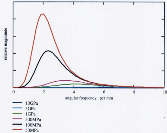
Figure 5.18. Plot of curvature spectrum of point-load mode-scrambler with dual-coated fibre, for a range of Young's modulus of the jaw.
