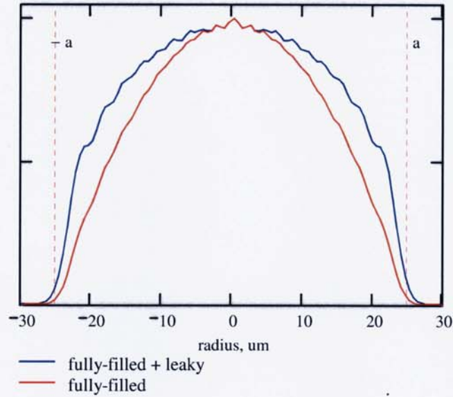
Figure 3.12. Computed near-field intensity profile of 50µm graded-index fibre showing guided modes (red) and effect of adding leaky modes to guided modes (blue).
