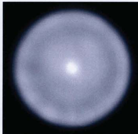
Figure 5.27. Near-field image of step index fibre with air gap mode-filter for 1000um gap width.
