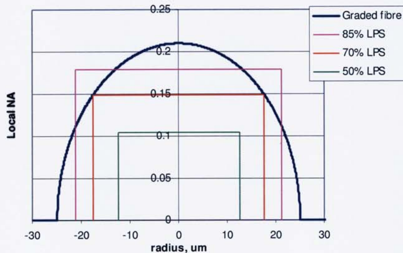
Figure 6.4. Local NA of graded-index fibre and several LPS launches. The diameter and NA of the graded fibre were 50um and 0.21, respectively.
