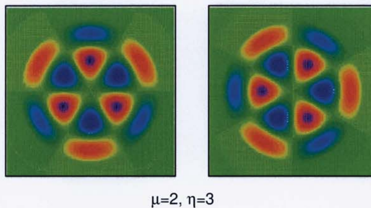
Figure 3.4. Field plots of two degenerate forms of LP_{3,2} mode in step-index fibre.
