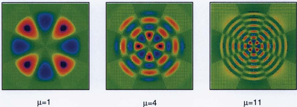
Figure 3.2. Examples of field distributions for modes in step-index fibre having azimuthal mode number \eta=4 and different radial mode numbers, \mu .
