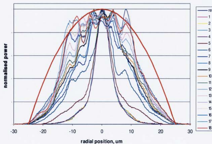
Figure 5.13. Near-field profiles of a 50 \mu m graded-index fibre with refractive-index grating vs number of exposures. The red curve represents a fully-filled distribution.
