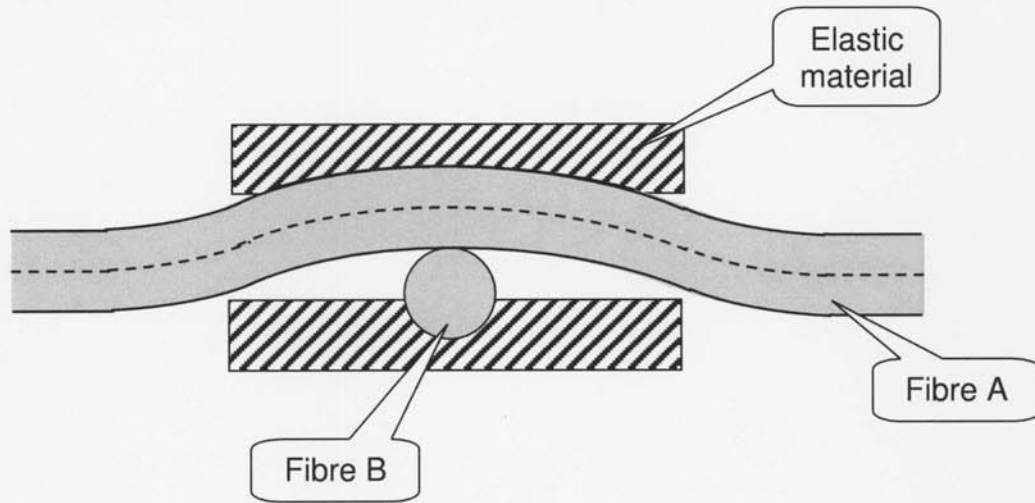
Figure 5.15. Schematic of crossover point in single loop mode-scrambler with silica fibre and elastic compression jaws.
