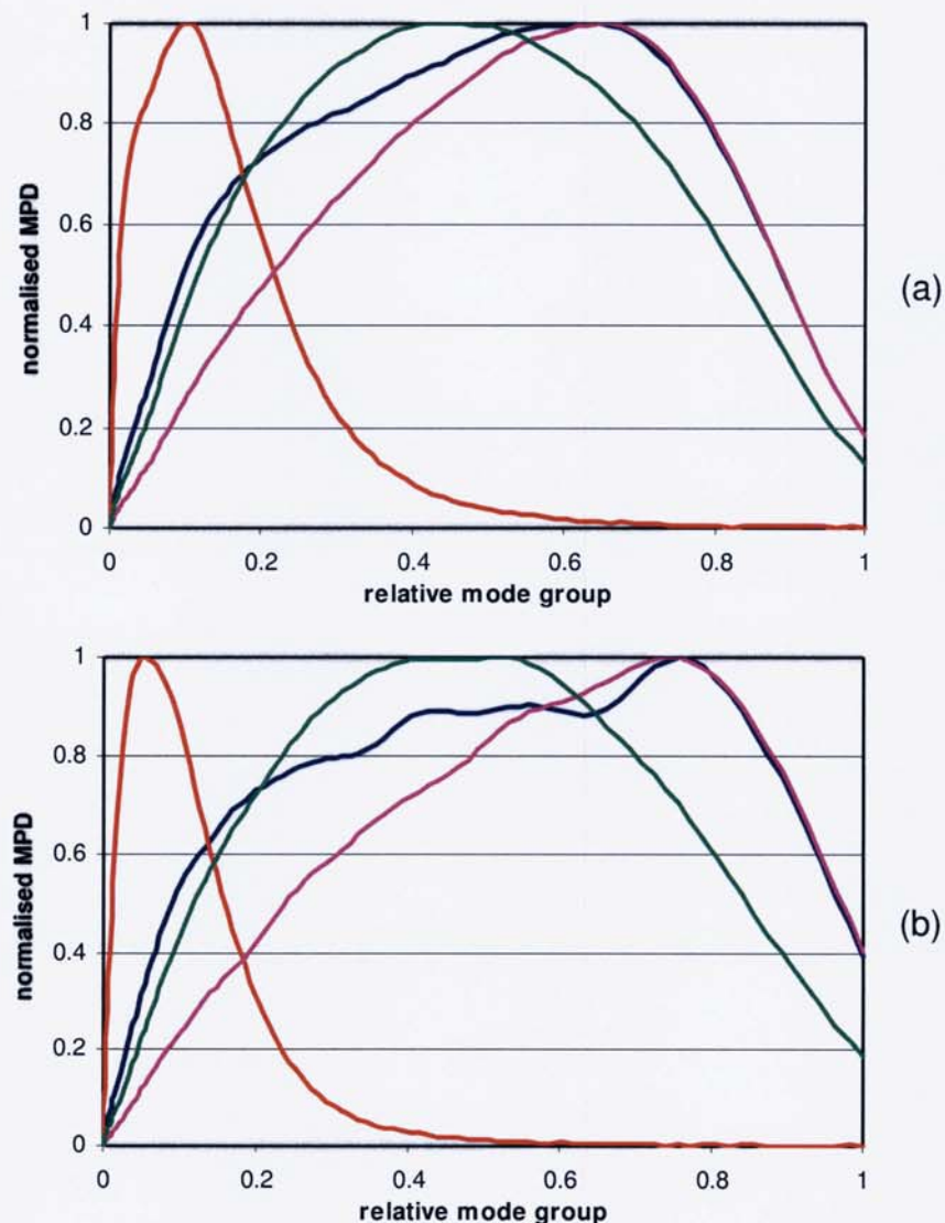
Figure 2.1. Plots of normalised MPD in a length of 62.5um tight-buffered fibre cable after (a) 202m, and (b) 1m
