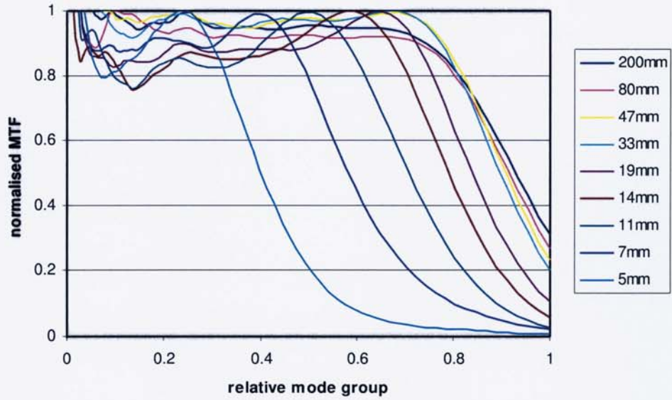
Figure 5.33. MTF of 50um graded-index fibre vs bend diameter of single-turn mandrel-wrap mode-filter.
