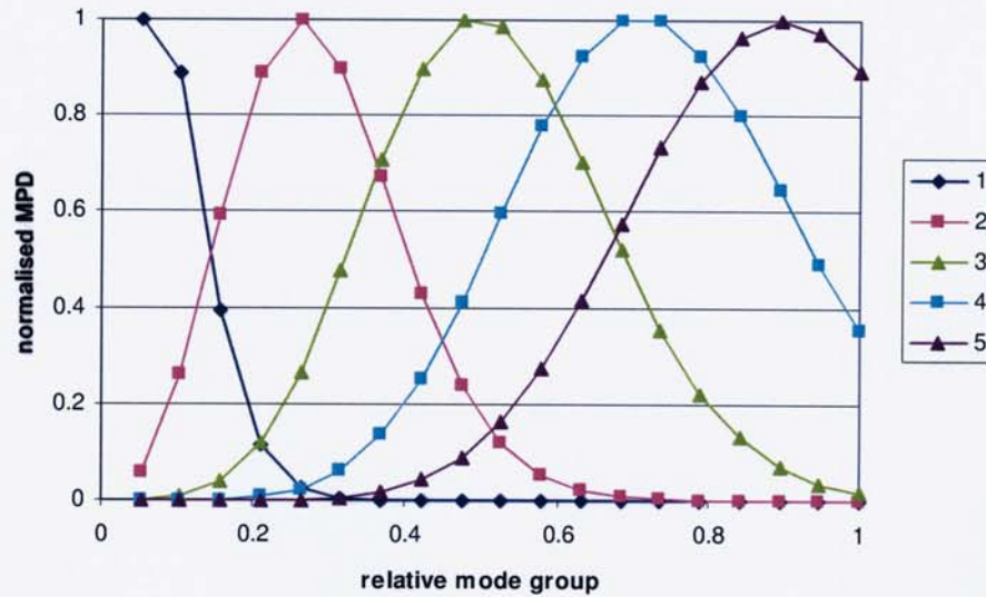
Figure 5.6. Computed MPDs for 7 pin microbend grating for grating amplitudes from 1.1 \mu m (curve 1) to 4.8 \mu m (curve 5).
