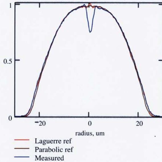
Figure 4.25. Computed near-field intensity profiles of 50µm graded-index fibre using Laguerre reference (red) and parabolic reference (brown). The measured profile is shown in blue.
