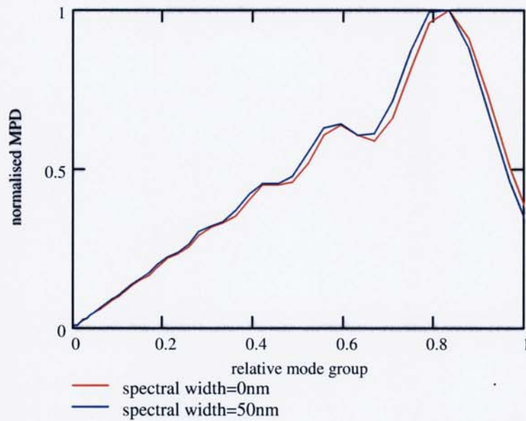
Figure 6.18. Normalised MPD of theoretical near-field of parabolic index fibre at 850nm as a function of spectral width.
