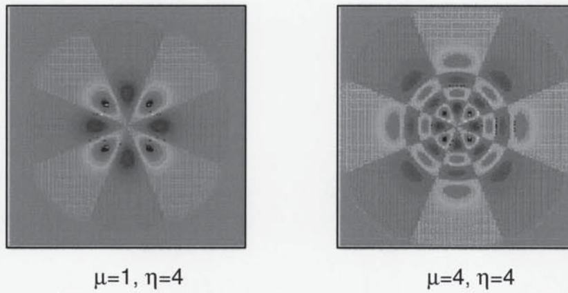
Figure 3.6. Examples of field distributions for modes in parabolic-index fibre having azimuthal mode number \eta=4 and different radial mode numbers, \mu .
