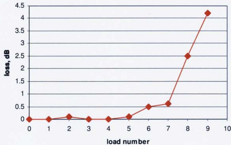
Figure 5.3. Insertion loss of a 50um graded-index fibre in a microbend grating as the load is increased.
