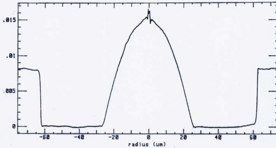
Figure 4.27. Refractive index profile of 50 \mu\text{m} graded index fibre.
