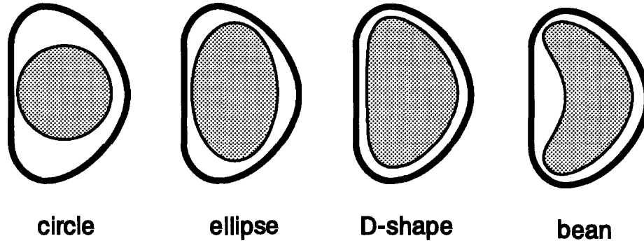
Figure 2: Cross-sections of the COMPASS vacuum vessel showing some examples of potential plasma shapes. The solid curve is the boundary of the vacuum vessel, and the plasma is shown by the shaded regions.
