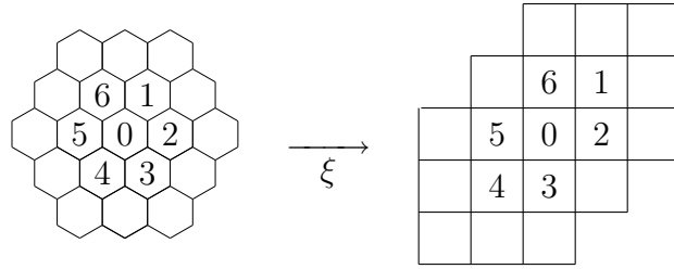
Figure 3: From the hexagonal to the square grid
