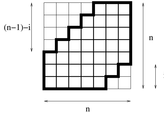
Figure 4: The region S_i(n)
