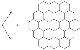
Figure 1: A Lee sphere, and three natural directions
