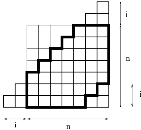
Figure 6: A triangular board covering \pi
