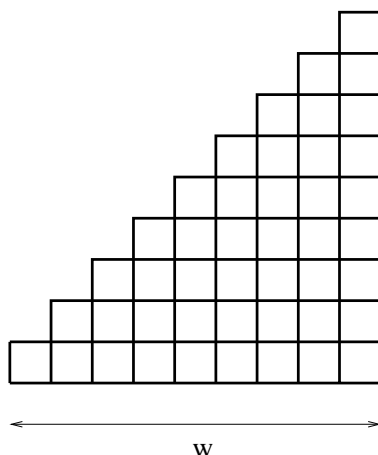
Figure 5: A triangular board of width w
