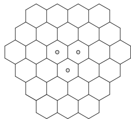
Figure 2: A tricentred Lee sphere
