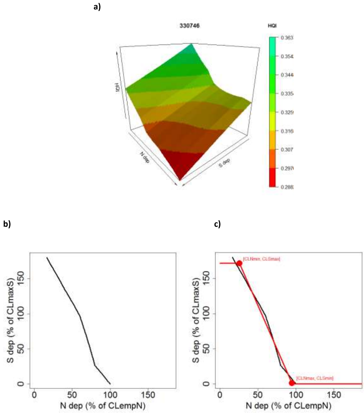
Figure 6.3: Response of habitat quality of an acid grassland Special Area for Conservation, Hill of Towanreef, to nitrogen (N) and sulphur (S) deposition scenarios: a) response illustrated in a '3D' plot; b) combinations of N and S deposition resulting in a critical value for habitat quality, HQI_{crit} ; c) simplified version of the HQI_{crit} response function.
