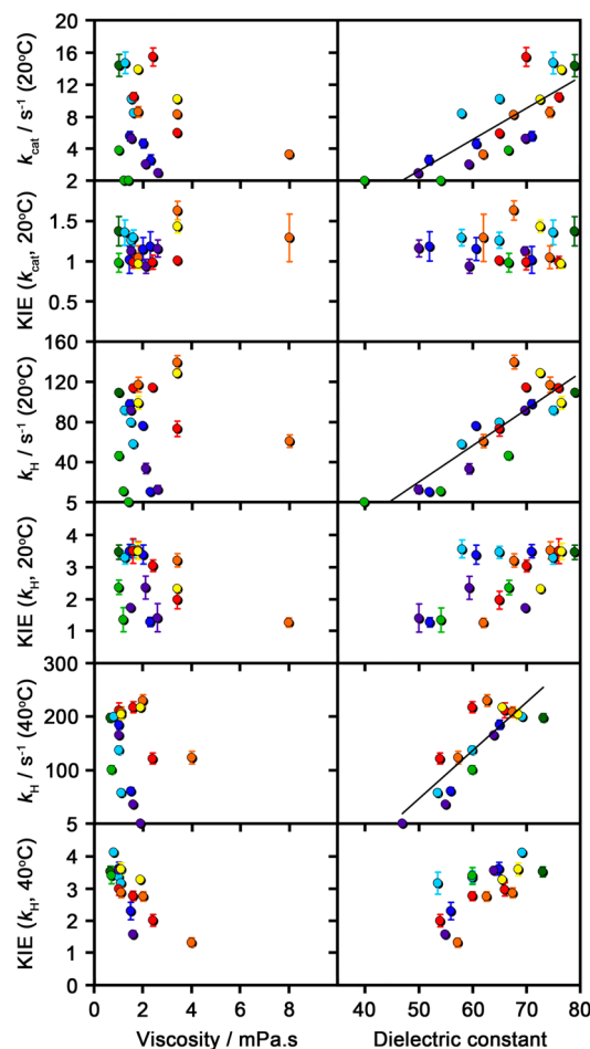
Figure 6. Plots of k_{cat} , k_H and their KIEs against solution viscosity (left) and dielectric constant (right). Symbols represent the different cosolvents, where green denotes no cosolvent, light blue methanol, dark blue ethanol, purple 2-propanol, red ethylene glycol, orange glycerol, yellow sucrose, and light green THF. In the case of dielectric constant data, lines of best fit are shown.
