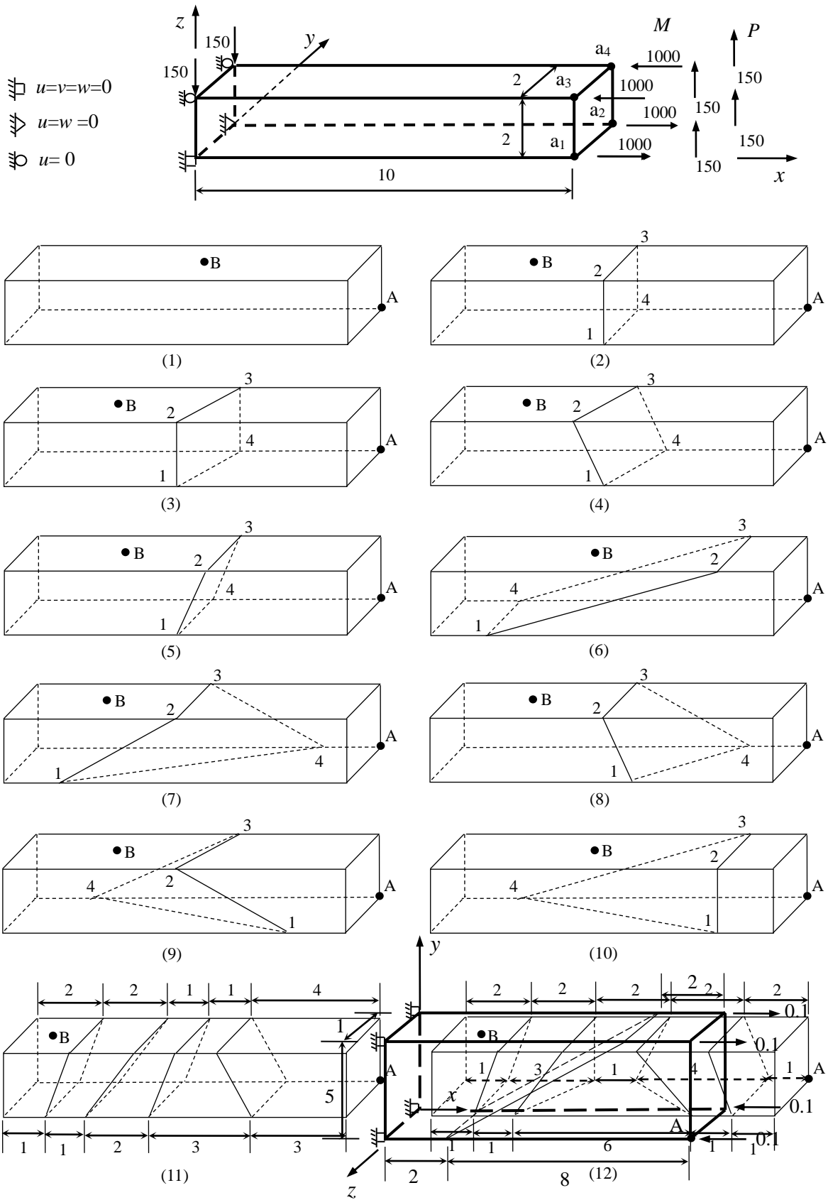
Figure 4. Cheung and Chen beam tests. E=1500 ; \mu=0.25
