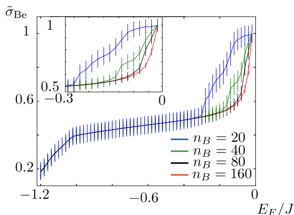
Figure C.2. Plot of the numerically estimated Berry conductivity \tilde{\sigma}_{Be} with error bars for four different values of the discretization number of the momentum space grid, n_B = 20, 40, 80 and 160 , for a system with parameters J_2 = 0.1J , \beta = 0.5J and n_R = 20 . The inset shows a zoom into the region -0.3J \leq E_F \leq 0 .
