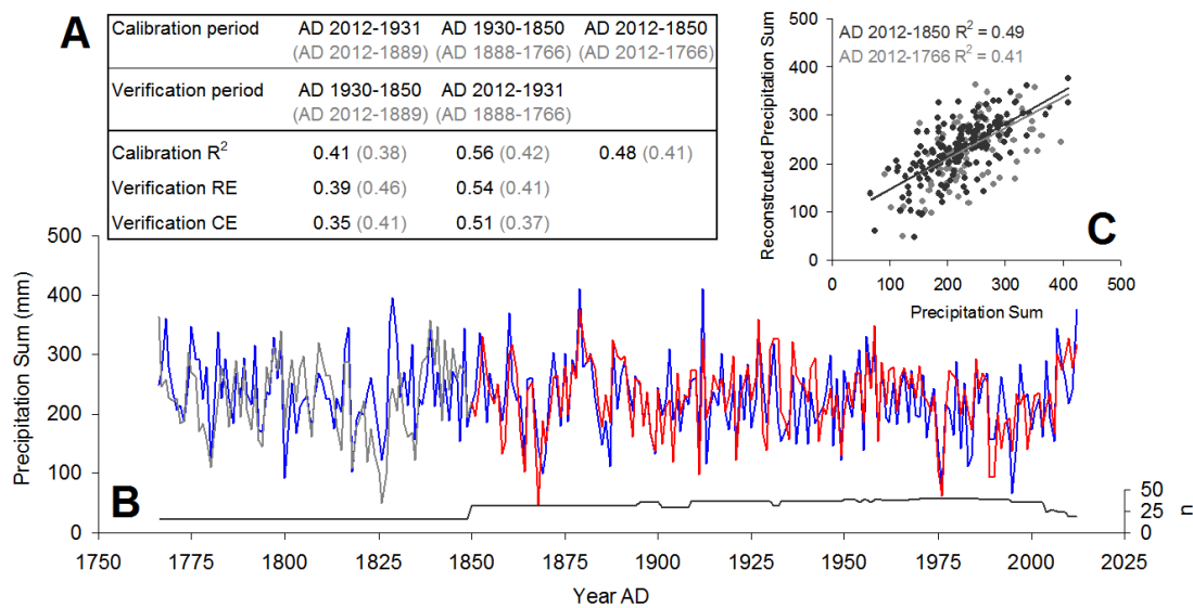
Fig. 5: Composite figure showing calibration and verification of the oak \delta^{18}\text{O} composite reconstructing summer England and Wales precipitation (EWP) over two periods: period 1 (AD 1850 to 2012) of good replication; and period 2 (AD 1766 to 2012, covering the entire summer EWP), including the period of lower replication from AD 1766-1849. Panel A shows calibration and verifications statistics: period 1 (black type) period 2 (grey type). Panel B shows inverted oak \delta^{18}\text{O} composite, AD 1850-2012 (red line), extended to AD 1766 (grey line), scaled to summer EWP (blue line). Panel C shows a scatter plot of summer EWP against \delta^{18}\text{O} composite scaled to summer EWP (black dots), filled grey circles and caption show the period AD 1766 to 1849.
