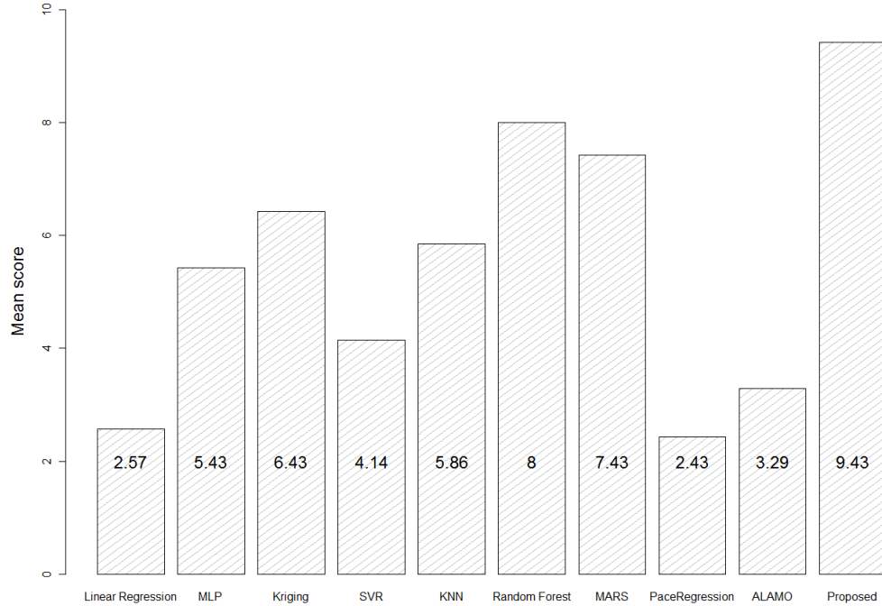
Figure 5: Scoring of regression methods
