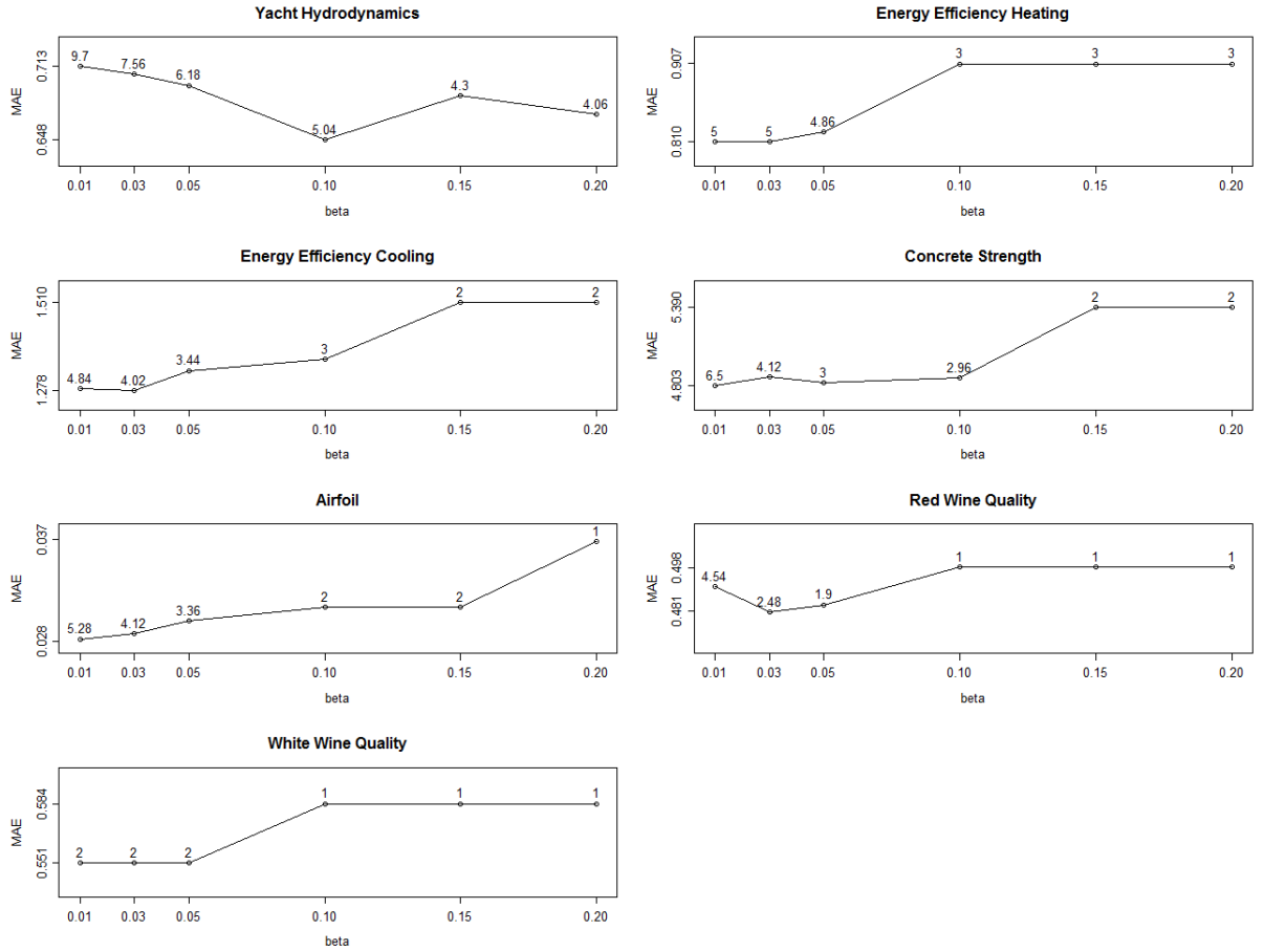
Figure 4: Sensitivity analysis of \beta . The numbers above points in each plot correspond to the average numbers of final regions.
