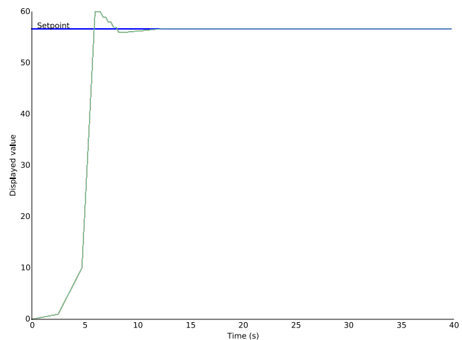
Fig. 14. Entering a large set point (56.7) with 33 iterations of simulation; no simulated delay or noise.
