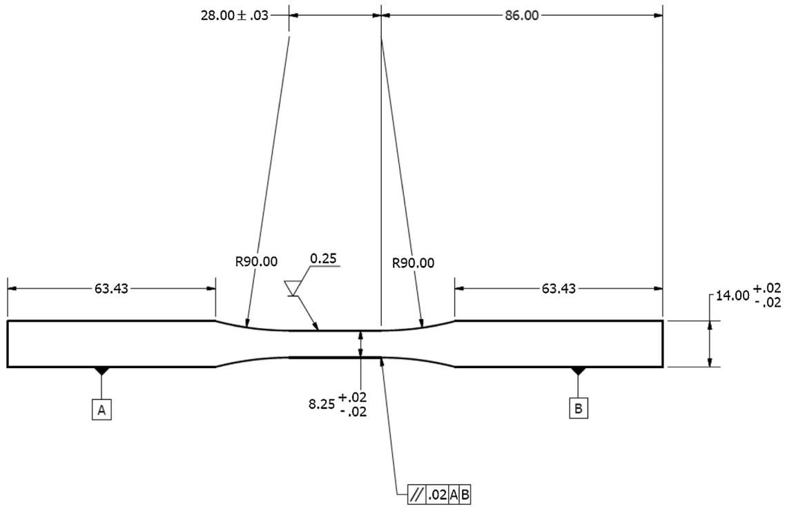
Fig. 1. Specimen design.
