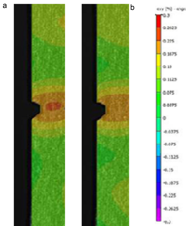
Fig. 14. Stress relaxation at a notch feature under monotonic tensile loading (image A followed by B).
