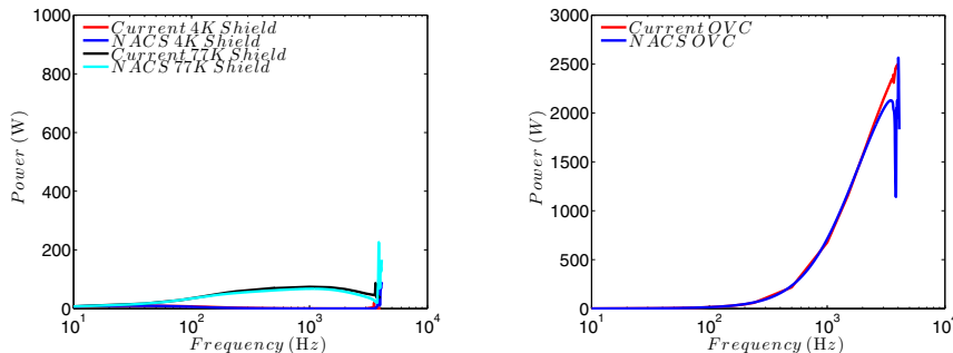
Figure 5: Comparison of the Ohmic power in the 4K shield, 77K shield and OVC obtained using our fixed point algorithm using a discretisation with uniform p = 1 elements and that obtained with NACS.
