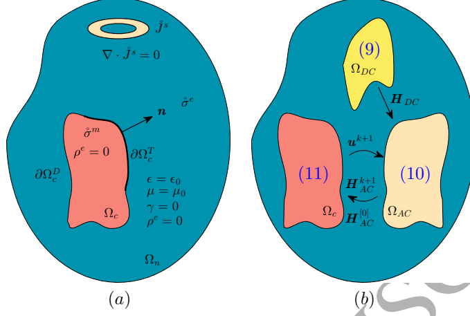
Figure 2: Geometrical description of coupled magneto-mechanical model, a) A fully coupled problem, b) Algorithmic idealisation
