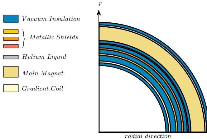
Figure 1: Radial Cross-section of a Simple MRI Scanner
