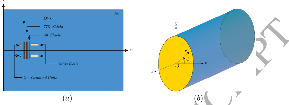
Figure 3: Simplistic MRI scanner in an axisymmetric geometry; (a) is a longitudinal sectional cut of (b).
