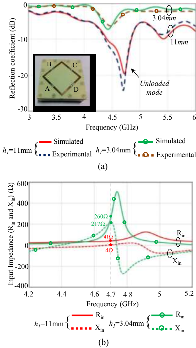
Fig. 2. (a) Reflection coefficients, ( inset ) prototype and (b) Input impedances of the conventional SLA simulated for different substrate thickness h_l .
