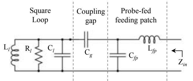
Fig. 4. Equivalent circuit model of CCSLA
