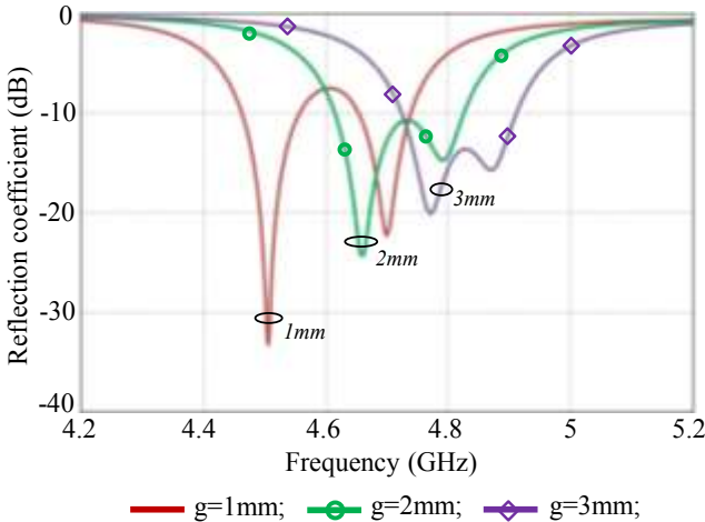
Fig. 8. Effect of the gap length on the reflection coefficient of the CCSLA.
