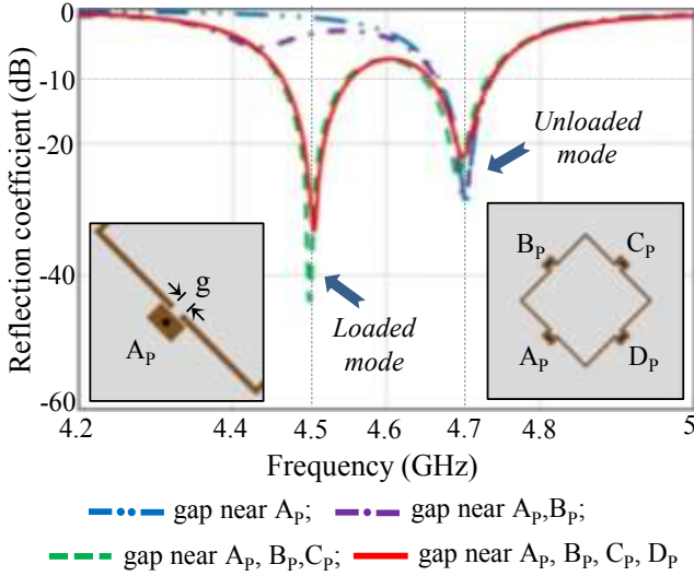
Fig. 7. Reflection coefficients of the CCSLA with loaded gap cut at different positions in the square loop.
