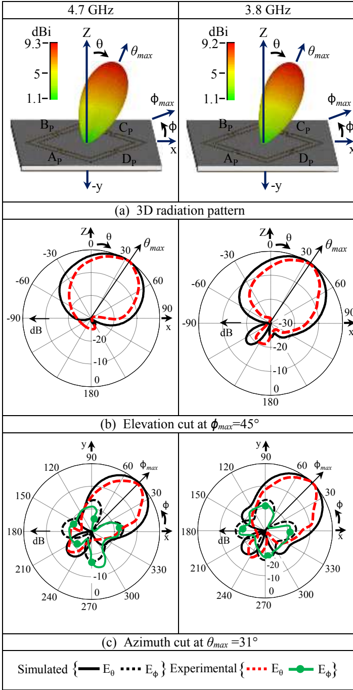
Fig. 11. Simulated and experimental radiation patterns of DBCCSLA at 4.7 GHz and 3.8GHz (a) three-dimensional, (b) elevation cut at \phi_{max} = 45^\circ and (c) azimuth cut at \theta_{max} = 31^\circ .
