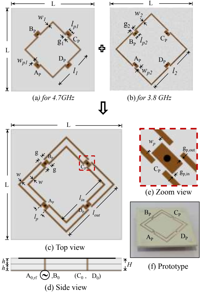
Fig. 9. (a) Top view of the CCSLA operating at 4.7 GHz. (b) Top view of the CCSLA operating at 3.8 GHz. (c) Top view of the DBCCSLA. (d) Side view of the DBCCSLA. (e) Zoom view of capacitively coupled feeding section. (f) Fabricated prototype of the DBCCSLA.
