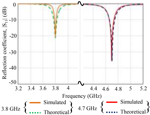
Fig. 5. Simulated and theoretical reflection coefficients of CCSLA for the two dimensions given in Table. 1
