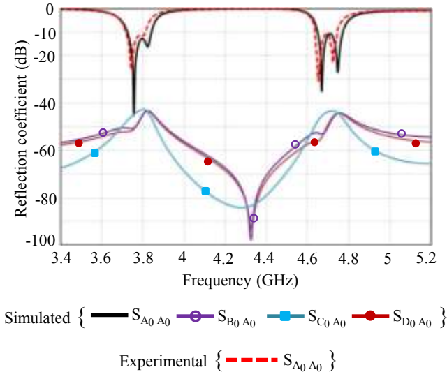
Fig. 10. Simulated and experimental reflection coefficient of the DBCCCLA.
