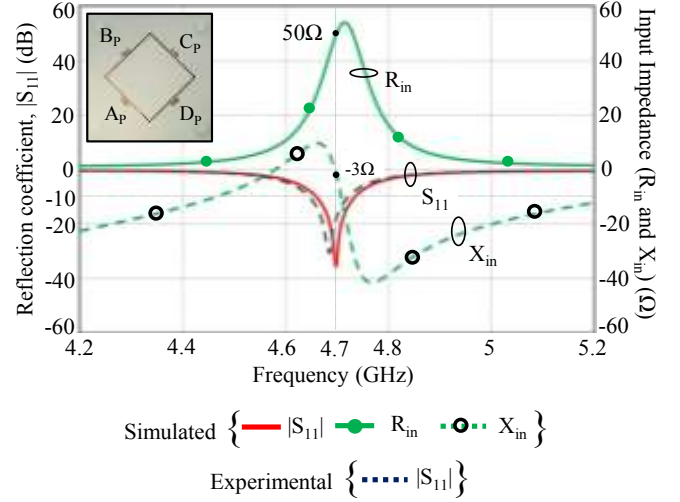
Fig. 6. Reflection coefficients and input impedances of the CCSLA for substrate thickness H=3.04 mm. (inset) prototype.
