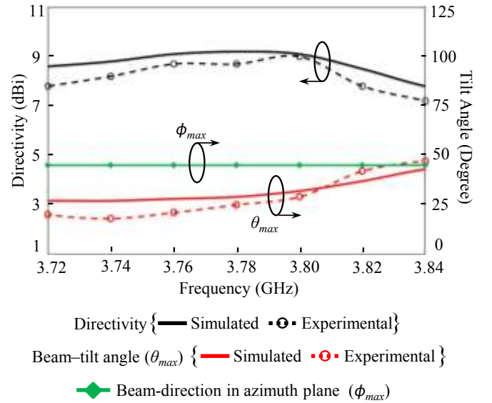
Fig. 13. Simulated and experimental beam-tilt angle and directivity of the antenna in the direction of the maximum radiation over the 3.8 GHz (3.72-3.84 GHz) frequency band.
