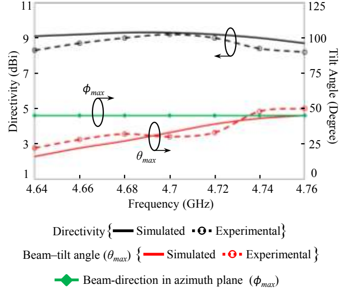
Fig. 12. Simulated and experimental beam-tilt angle and directivity of the antenna in the direction of the maximum radiation over the 4.7 GHz (4.64-4.76 GHz) frequency band.
