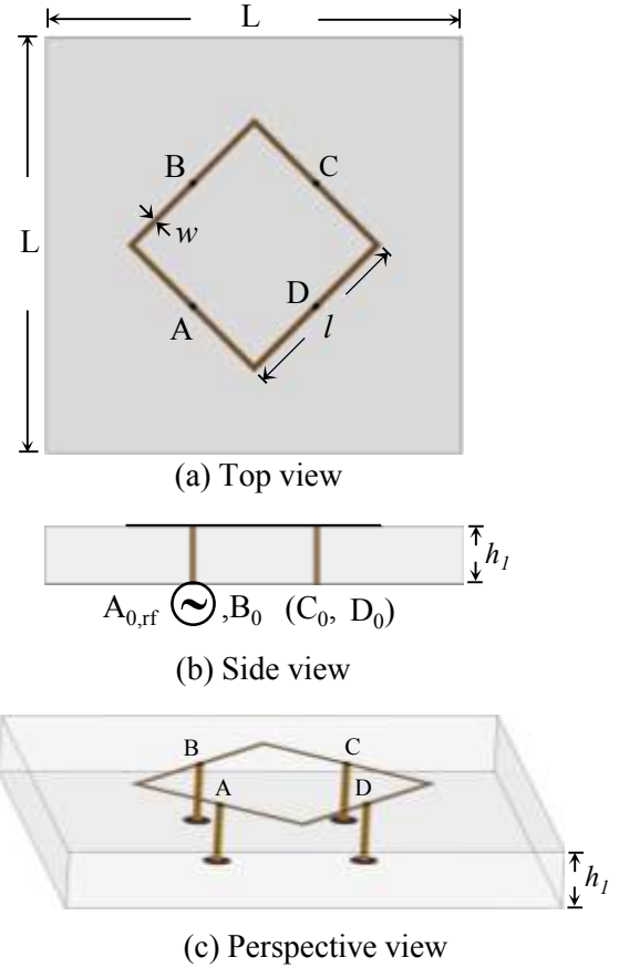
Fig. 1. Top, side and perspective views of the probe fed square loop antenna (SLA).
