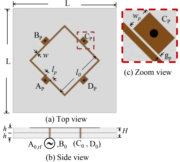
Fig. 3. Top, side and zoom views of the single loop CCSLA with a substrate thickness of 3.04 mm.
