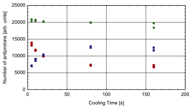
Fig. 18. Electron cooling of antiprotons. The electron plasma was comprised of 20 million particles with a radius of 0.55 mm. The uncooled antiprotons are those released when the high voltage is switched off, leaving only those which have fallen into the trap well containing the cold electrons. ● Uncooled, ■ Cooled, ◆ Total Number.
