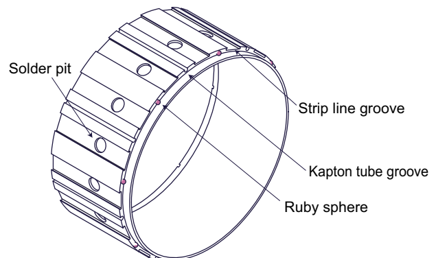
Fig. 5. Illustration of a single mixing trap electrode. The wall thickness is 1.5 \text{ mm} , the inner diameter is 44.5 \text{ mm} and the signal runs in strip-lines soldered to the relevant electrode.
