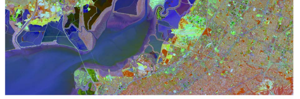
PCA, \gamma = 0.795
