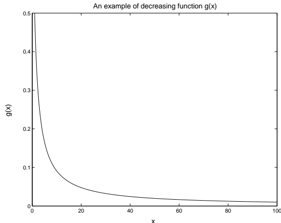
Figure 1.2: Plot of the monotonically decreasing function g(x) = 1/(1+x) .
