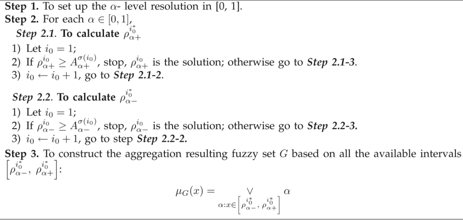
Fig. 1. Procedure of the Alpha-Level Approach to type-1 OWA operation.
