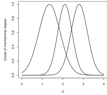
Fig. 2. Three aggregated fuzzy sets (from left to right): A^1 , A^2 , and A^3 .
