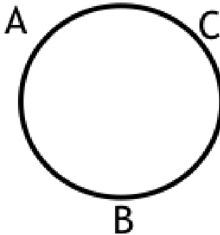
Figure 3: The round table problem
