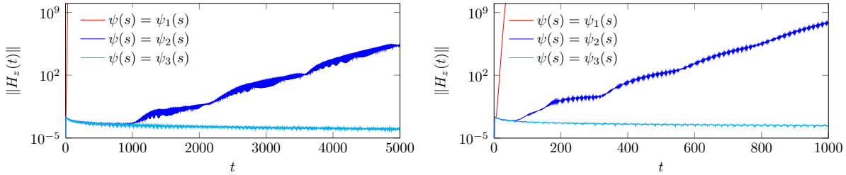
FIGURE 8. The dependence of the L^2 -norm of the solution H_z (computed inside the domain and the PML) to the problem of Example 5.24 on time, computed with different PMLs. In the left plot \nu = 0.01 in (85), and in the right plot \nu = 0.1 .
