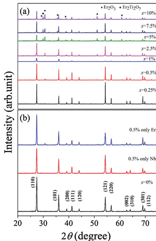
Fig. 1 XRD patterns of (Er 0.5 Nb 0.5 ) x Ti 1-x O 2 sintered ceramics: (a) x = 0.25\% , 0.5%, 1%, 2.5%, 7.5% and 10%, (b) x = 0\% , 0.5% only Nb and 0.5% only Er.
