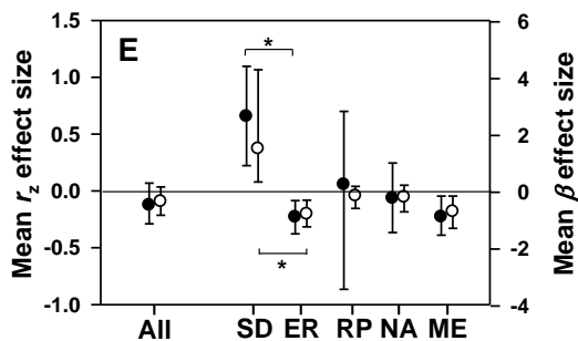
Figure 3. Mean effect size ( \pm 95\% CI) for overall effect, by habitat and by region of the relationship strength r_z (black circle) and slope \beta (open circle) between temporal variability and evenness J' . Effect sizes are displayed by type of analyses (species richness variability: A, B; community assemblage variability in: structure C, D and composition E, F) and scale of evenness measure (average by patch scale as Quadrat: A, C, E; reassessed by shore as Site: B, D, F). See Figure 2 for abbreviations.
