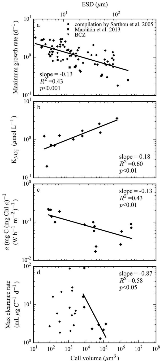
Fig. 1. Size dependency of major diatom functional traits: (a) \mu_{\max} (review by Sarthou et al. 2005 and additional data from Marañón et al. 2013; V. Rousseau and J.-Y. Parent pers. comm. for the BCZ); (b) K_{\text{NO}_3^-} (review by Litchman et al. 2007); (c) \alpha (data from Taguchi 1976); and (d) \text{aff}_{\text{DA}}^{\text{CP}} estimated from the maximum clearance rate of copepods on prey of different sizes (review by Gismervik et al. 1996). The allometric relationship for \text{aff}_{\text{DA}}^{\text{CP}} is estimated from data above the optimal prey size ( \sim 3 \times
