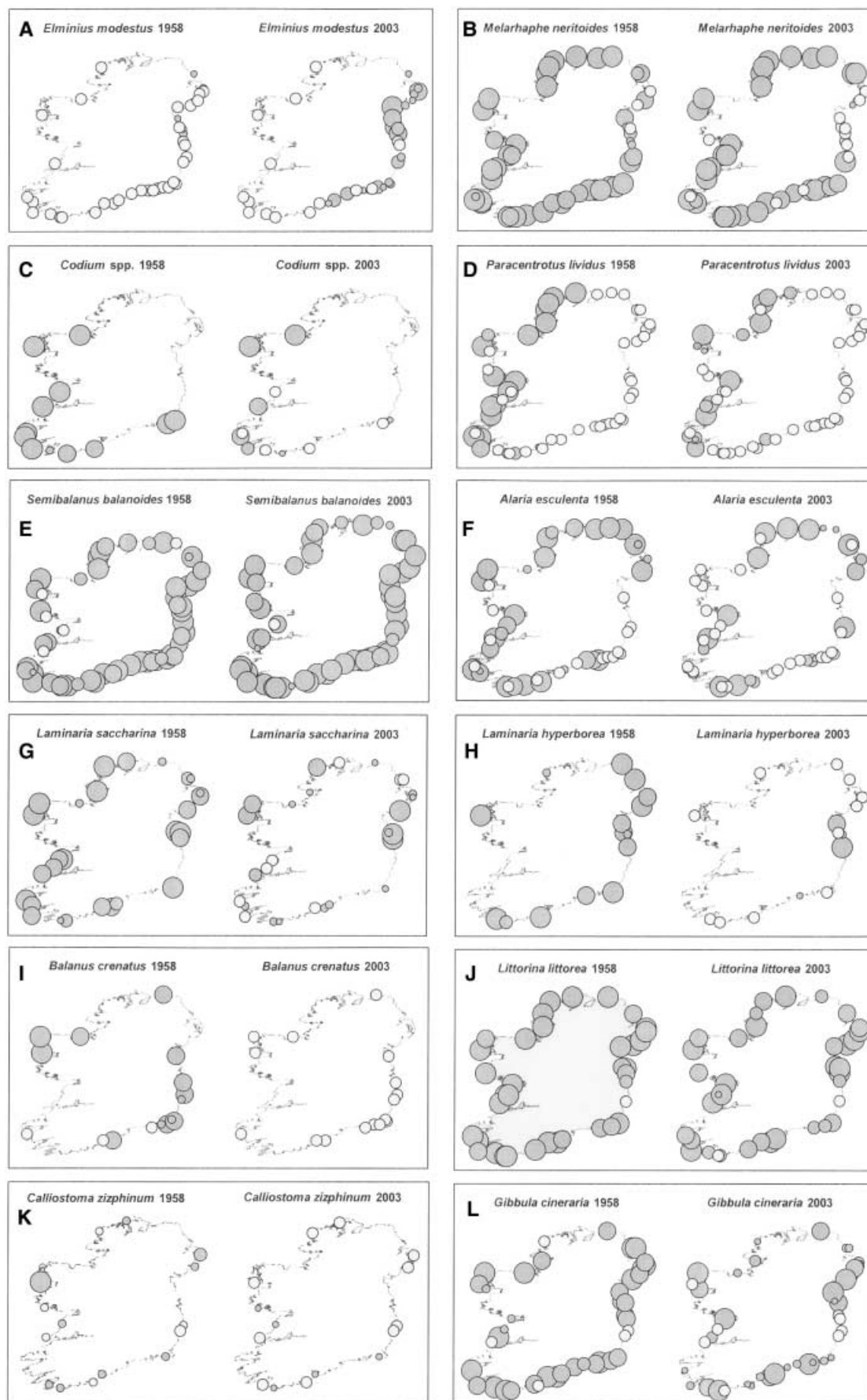
Figure 2. (A–L) The distribution and abundance (using the ACFOR scale) of 12 species that showed a significant change in abundance between 1958 and 2003 (based only on shores that were sampled during both surveys). ○, Not seen, ◊, Rare; ◐, Occasional; ◑, Frequent; ◒, Common; ◓, Abundant.
