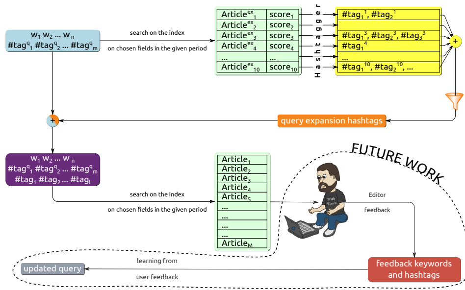
Figure 4: Story retrieval process diagram.
