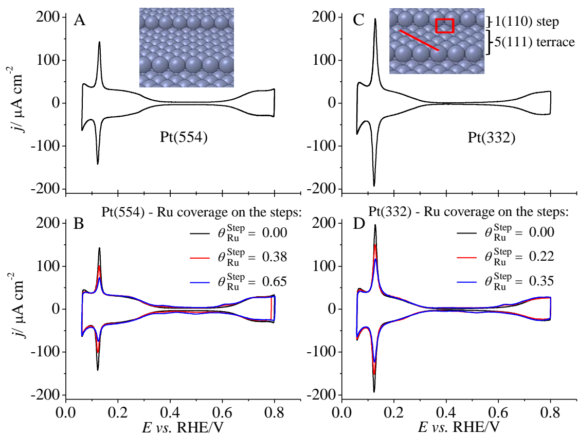
Fig. 1. Cyclic voltammograms of two stepped Pt electrodes before (A and C) and after (B and D) selective modifications of their steps by Ru. Data recorded at 0.05 \text{ V s}^{-1} in 0.1 \text{ M HClO}_4 . Data includes hard sphere models of the stepped surfaces.
