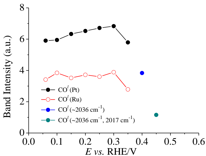
Fig. 9. Integrated band intensities for adsorbed CO on sites of Pt and Ru for a Ru modified Pt(332) electrode ( \theta_{\text{Ru}}^{\text{Step}} = 1.0 plus \theta_{\text{Ru}}^{\text{Terrace}} \simeq 0.35 ). Data extracted from the Figure 8.
