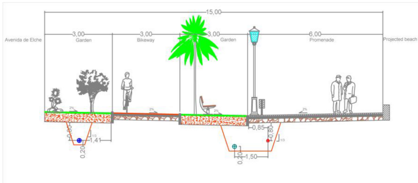
Figure 5: Main cross-section.
