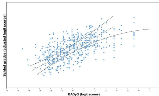
Figure 2. Person logit school grades plotted against person logit Badyg scores in the second course of ESO, with 95% confidence bands
