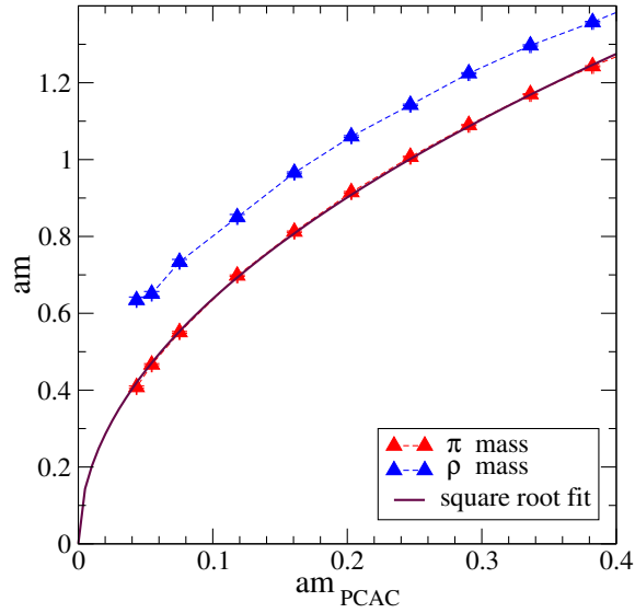
Figure 1: The hadron masses at N_f = 2 with \beta = 1.0 . The square root behaviour of the pseudoscalar is evident.
