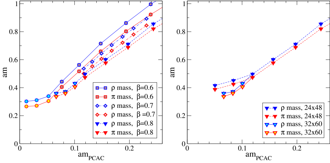
Figure 3: Left: Pion and rho masses in N_f = 6 with \beta = 0.6, 0.7 and 0.8 . The points with yellow center refer to the bigger lattice size. Right: The effect of the lattice size on the hadron masses with \beta = 0.8 .
