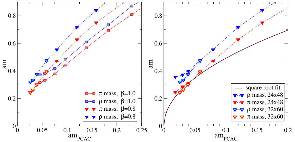
Figure 2: Left: Pion and rho masses at N_f = 4 with \beta = 1 and 0.8 . The points with yellow center refer to the bigger lattice size ( 32^3 \times 60 ). Right: the lattice size effect to the hadron masses at \beta = 0.8 .
