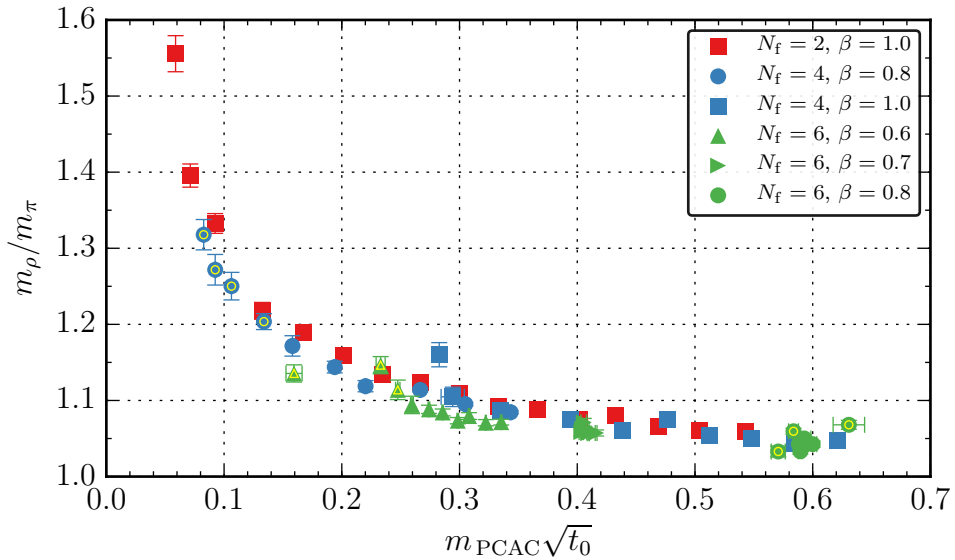
Figure 5: Results in physical units. The results are observed to settle on a universal curve; the underlying reason for this scaling is currently unclear.
