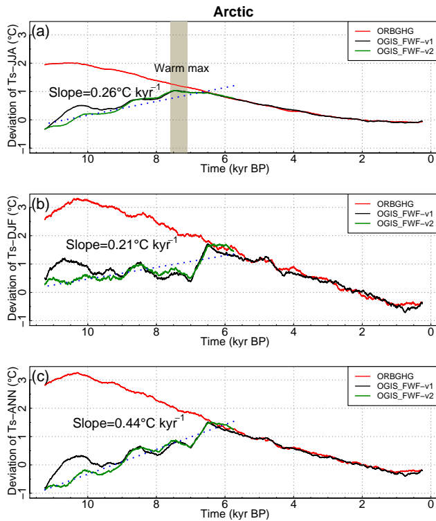
Figure 4. Simulated temperature evolution, shown as the anomalies compared to PI, since the early Holocene at high latitudes (north of 70°). Panels (a), (b) and (c) represent the summer, winter and annual values, respectively. The slope indicates the overall warming rate and is based on the least-squares regression over the period from the 11.5 to 6 kyr, as from 6 kyr the temperature starts to decrease. It is only a general estimation, and thus uncertainty ranges are not provided. The warmest peak is marked by a shaded bar and represents the simulated peak during which the temperature was over 1 °C higher than the PI. Both slope calculation and warm peak are based on the OGIS_FWF-2 simulation.
