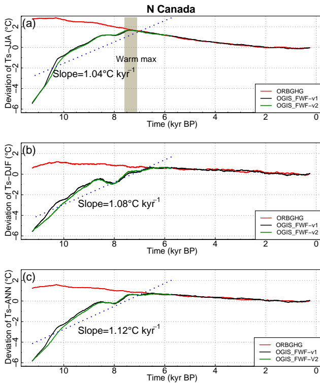
Figure 6. Same as Fig. 4 but for northern Canada (120–55° W, 50–69° N).
