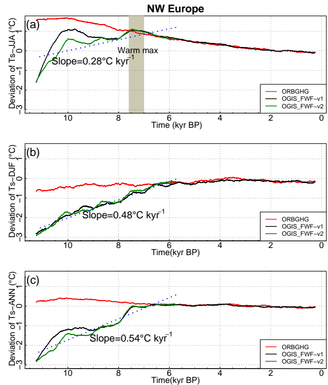
Figure 5. Same as Fig. 4 but for northwestern Europe (5° W–34° E, 58–69° N).
