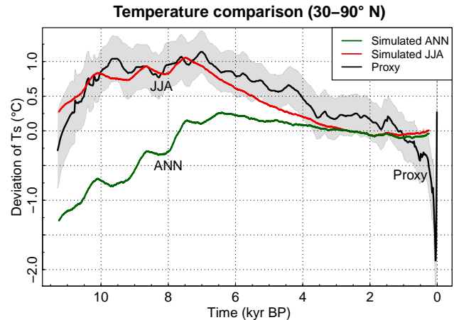
Figure 9. Model–data comparison over the latitudinal band of 30–90° N, shown as a deviation from the PI. The stacked temperature reconstruction with 1\delta uncertainty (grey band) is based on Marcott et al. (2013).
