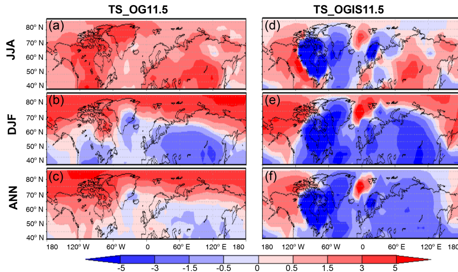
Figure 3. Simulated temperatures for 11.5 kyr, shown as deviation from the PI. Left column shows the simulation with only GHG and ORB forcings (OG11.5). For the right column, the ice-sheet forcing is included (OGIS11.5). Upper, middle and lower panels present summer (JJA), winter (DJF) and annual mean temperatures, respectively.
