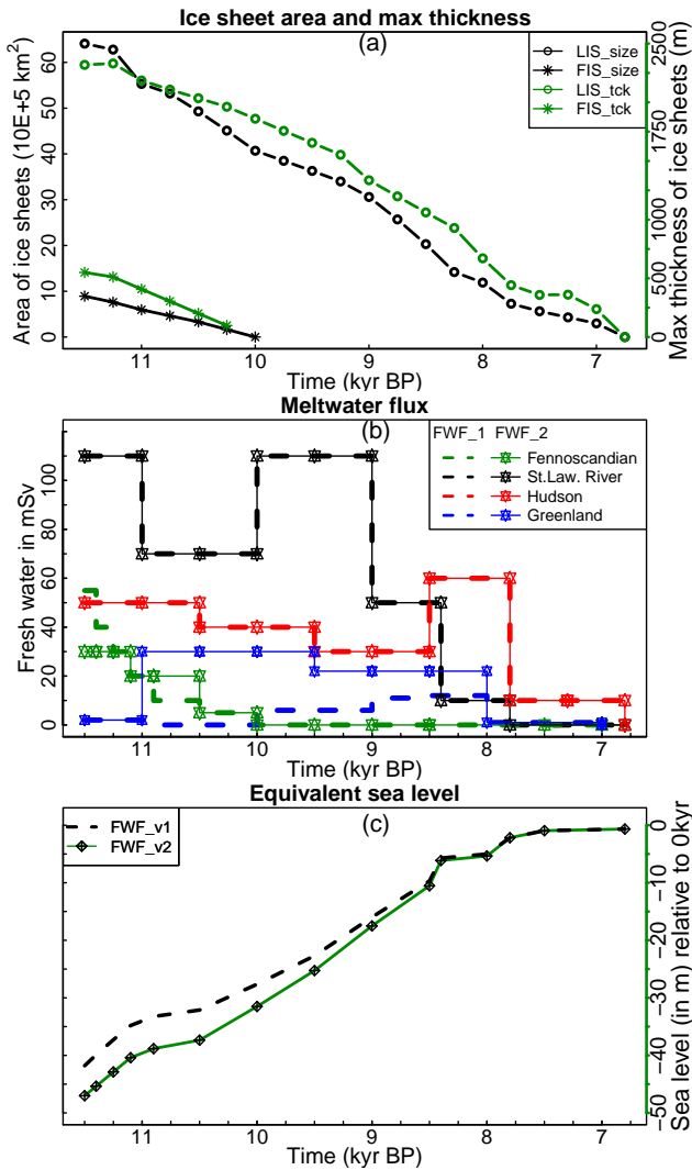
Figure 2. The prescribed ice-sheet forcing during the early Holocene. (a) Variation in ice-sheet extent ( \text{km}^2 ) displayed as the black lines with the axis on the left and their maximum thickness (m) indicated by the green lines with the axis on the right. A relatively minor change in GIS is not shown due to its small scale. (b) Two freshwater flux scenarios (in \text{mSv} ), FWF-v1 (thick dashed lines) and FWF-v2 (solid lines). (c) Total meltwater discharge in equivalent sea level (m).
