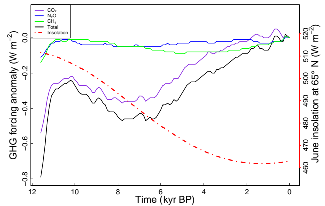
Figure 1. Evolution of greenhouse gas concentrations (GHGs) shown as the radiative forcing's deviation from the preindustrial level (with solid lines corresponding to the left axis), and June insolation at 65^\circ \text{N} derived from orbital configuration (with red line and the axis on the right).
