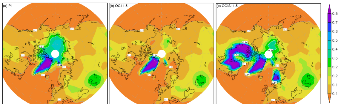
Figure 11. Summer surface albedo in the extratropical Northern Hemisphere. Panels (a), (b) and (c) represent the control run (PI) and the simulations without ice sheets (OG11.5) and with ice sheets (OGIS11.5), respectively.
