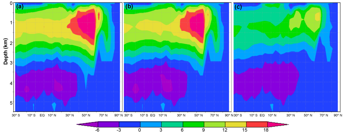
Figure 12. Meridional overturning stream function ( S_v ) in the Atlantic Ocean basin. Panels (a), (b) and (c) indicate the control run (PI) and the simulations OG11.5 and OGIS11.5, respectively. On the left-hand side, depth is indicated in kilometers. Positive values indicate a clockwise circulation. Maximum AMOC strength value was 22 S_v (reached at about 1200 m depth) in the PI and OG11.5 simulation, while it was only about 14 S_v (reached at 600–700 m depth) in OGIS11.5.
