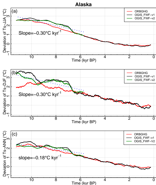
Figure 7. Same as Fig. 4 but for Alaska (170–120° W, 58–74° N).
