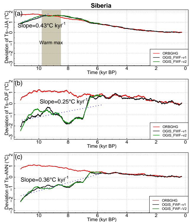
Figure 8. Same as Fig. 4 but for Siberia ( 62\text{--}145^{\circ}\text{E} , 58\text{--}74^{\circ}\text{N} ) and the warming rate slope is indicated for a shorter period (11.5–9.8 kyr).
