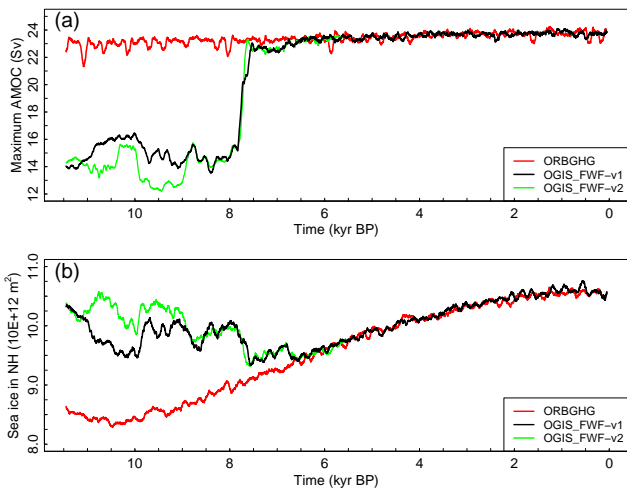
Figure 14. Response of the ocean variables (shown as a 100-year average) to forcings during the Holocene. (a) Maximum meridional overturning stream function (Sv) in the North Atlantic. (b) Sea-ice area ( 10^{12}\text{m}^2 ) in the Northern Hemisphere.
