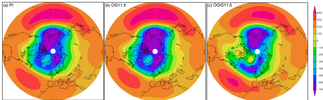
Figure 10. Geopotential height anomalies from global mean (in \text{m}^2 \text{s}^{-2} ) at 800 hPa in the extratropical Northern Hemisphere. Panels (a), (b) and (c) show the control condition PI and the simulations OG11.5 and OGIS11.5, respectively.
