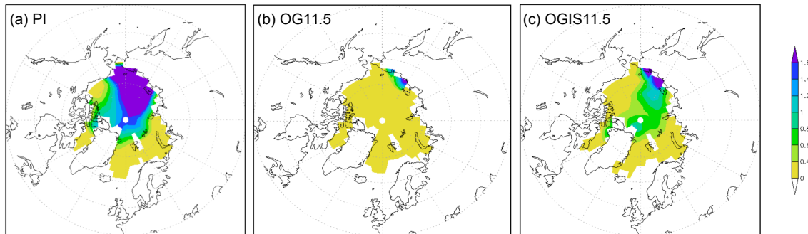
Figure 13. Minimum sea-ice thickness (m) in September for PI (a), OG11.5 (b) and OGIS11.5 (c).
